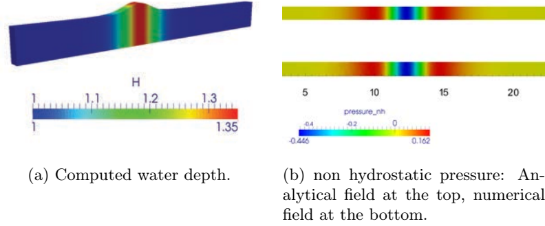
Figure 4.4: Illustration of the solitary wave propagation at t = 1.99s .
