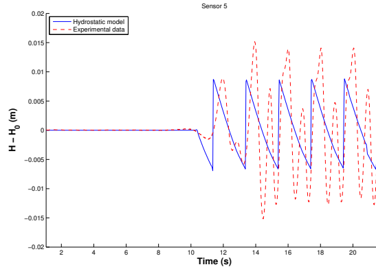
Figure 3.14: Comparison with hydrostatic model on sensor 5.
