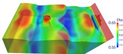
(e) Hydrostatic simulation at time t=9.59589 s
