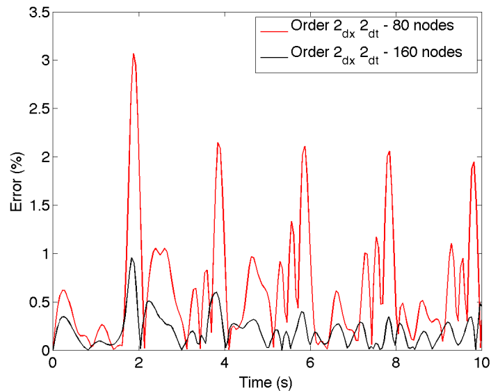
Figure 2.5: Parabolic bowl: variations along time of the error (2.124) at node x_0 = 0.8 m with 80 and 160 cells, 2^{nd} order scheme (space and time).
