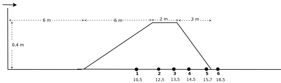
Figure 3.13: Configuration of Dingemans's test.
