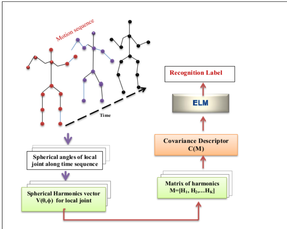
Figure 5.3: Overview of the calculation process of the proposed method. Firstly, we extract temporal spherical orientations of the joint . Then we represent these angels using SHS. Then we use covariance property to build the action descriptor on SHs. We apply ELM for recognition task
