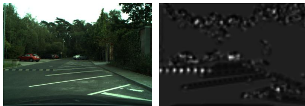
Figure 24: Example of how the appearance-based classifier works in the context-based object detection architecture: for each input image (a) , it produces a retinotopic, dense map of vehicle confidences (b) . This means that each pixel in this map represents the presence or absence of a vehicle, at a specific scale, centered on that pixel.
