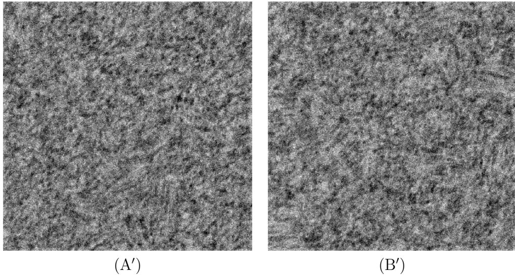
Figure 10.27: Simulated TEM images from (A') the identified two-scale model of platelets (B') the three-scale model of platelets for mesoporous alumina. The parameters of the microstructures are shown in Tab. 10.2.
