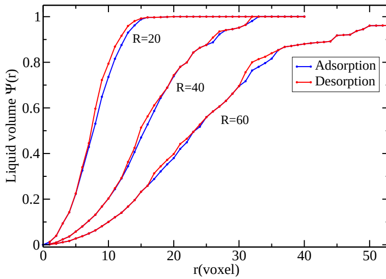
Figure 9.14: Capillary condensation (blue) and evaporation (red) isotherms of Boolean models of spheres, of increasing radius R = 60 voxels, R = 40 voxels and R = 20 voxels (bottom to top).
