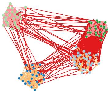
Final clustering
