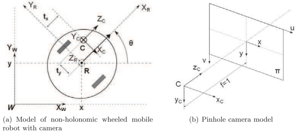
Figure 3.1: System modeling
