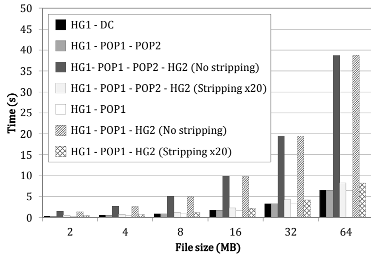
Figure 4.3: Read latencies. HG-DC : reading on the datacenter. HG1-POP1-POP2 : reading on the POP of a region different from the one where the request is issued. HG1-POP1-POP2-HG2 : reading on one HG connected to the POP of a region different from the one where the request is issued. HG1-POP1 : reading on the POP of a region from where the request is issued. No stripping : the object is read entirely in 1 HG. Stripping x20 : the 20 blocks stored in different HGs composing the object are read in parallel.
