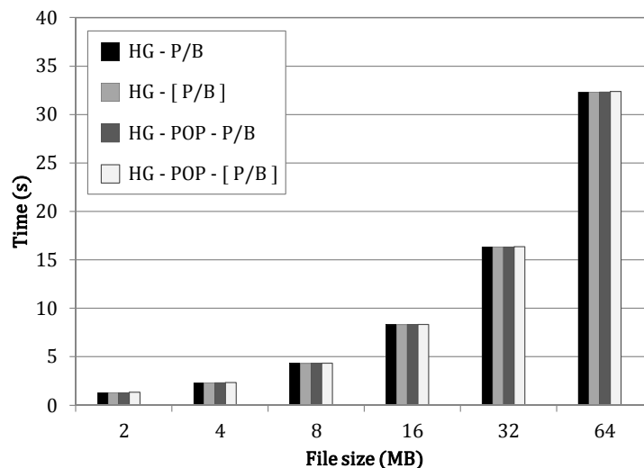
Figure 4.4: Write latencies in presence of crashes. See Figure 4.2 for meanings of HG-P/B and HG-POP-P/B . The element surrounded by brackets is the failed one. HG-[P/B] : writing from the primary POP region of an object and the primary or the backup POP is unavailable. HG-POP-[P/B] : writing of an object from a region different from its primary and backup regions while either the primary or the backup POP is unavailable.
