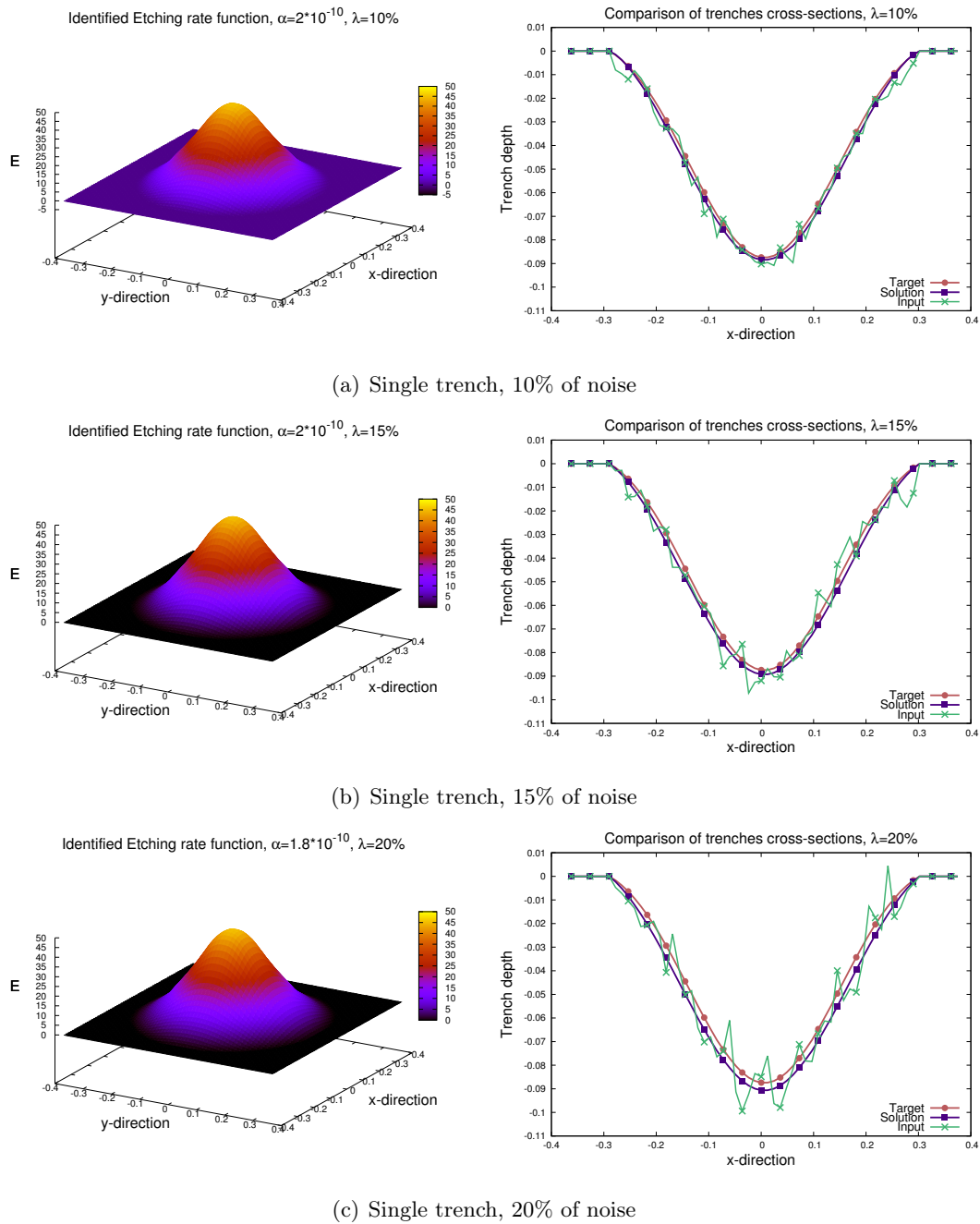
Figure 7.3: Results of numerical identification of the Etching rate functions for AWJM model and prediction of the surface shapes ("Solution") based on single trench measurement with applied noises of 10%, 15% and 20% respectively, compared with original trench profile ("Target") and noisy input ("Input").
