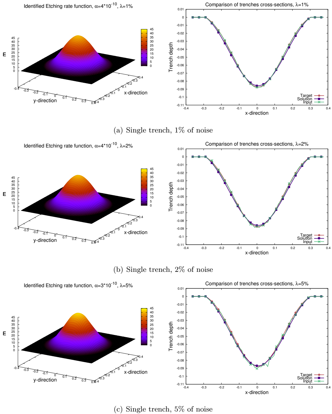
Figure 7.2: Results of numerical identification of the Etching rate functions for AWJM model and prediction of the surface shapes ("Solution") based on single trench measurement with applied noises of 1%, 2% and 5% respectively, compared with original trench profile ("Target") and noisy input ("Input").
