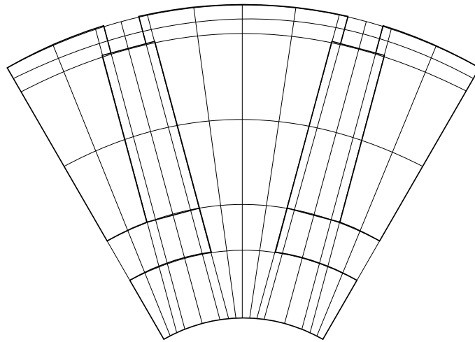
Fig. 3.11: Block mesh of the rotor
