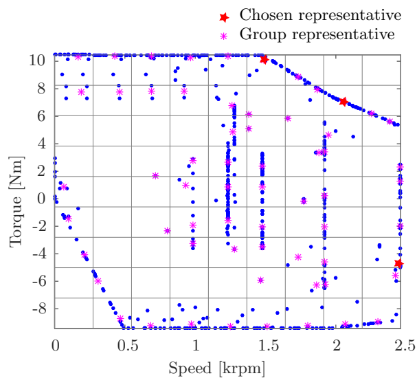
Fig. 5.20: Group division on the driving cycle space
