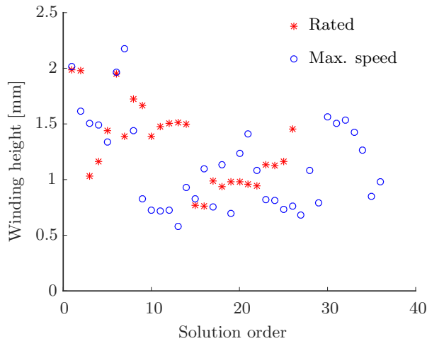
Fig. 5.14: Excitation winding height through solutions on the pareto front (From left to right in Fig. 5.13)
