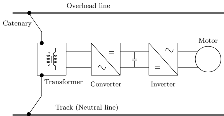
Fig. 1.3: Traction with electrification
