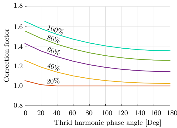
Fig. 3.36: Correction factor according to amplitude and phase angle of third harmonic
