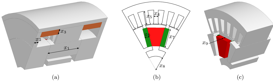
Fig. 5.9: Geometry variables
