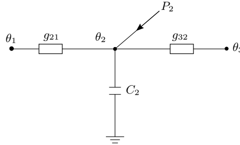
Fig. 4.14: A typical node in transient mode
