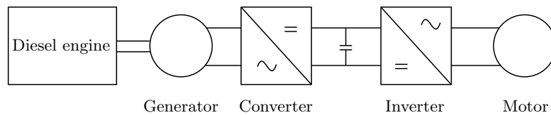
Fig. 1.2: Typical diesel electric traction system
