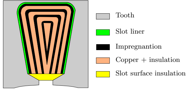
Fig. 4.10: Winding insulation in the slot
