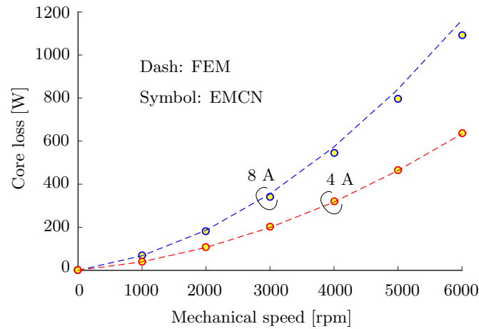
Fig. 3.48: Core loss according to load variation, I_{dc} = 0 A
