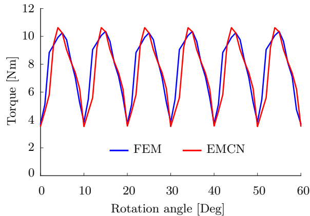
Fig. 3.31: Instantaneous electromagnetic torque at armature current of 8A, I_{dc} = 0 A
