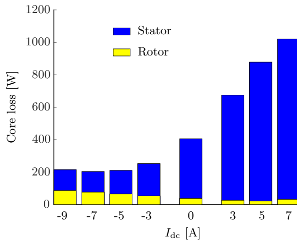
Fig. 3.44: Core loss by EMCN at 6000 rpm, no-load according to field current
