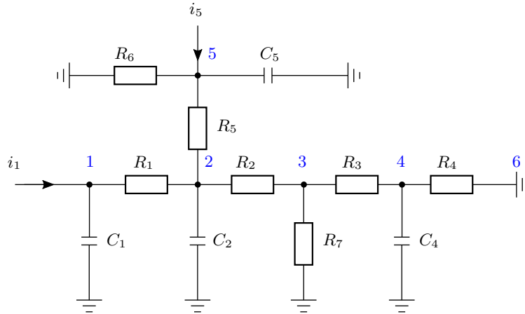
Fig. 4.16: A freely created R - C circuit with grounded capacitors
