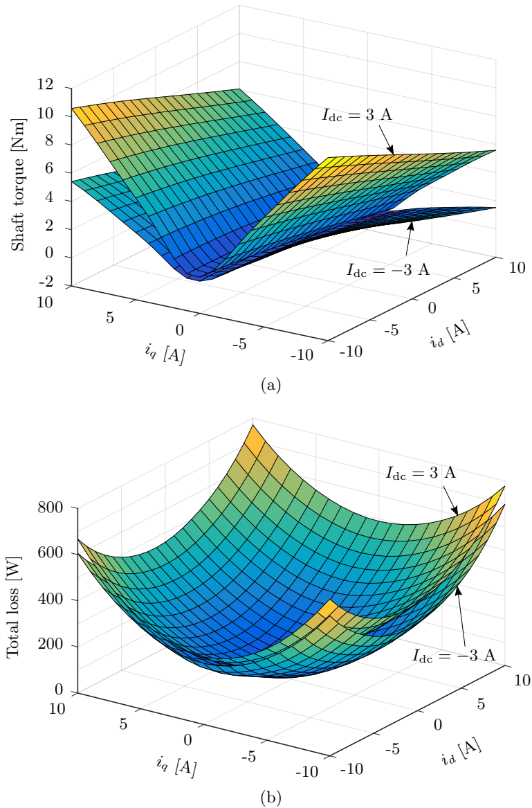
Fig. 5.3: Response surfaces at the speed 2000 rpm, motor mode. a) Shaft torque. b) Total loss
