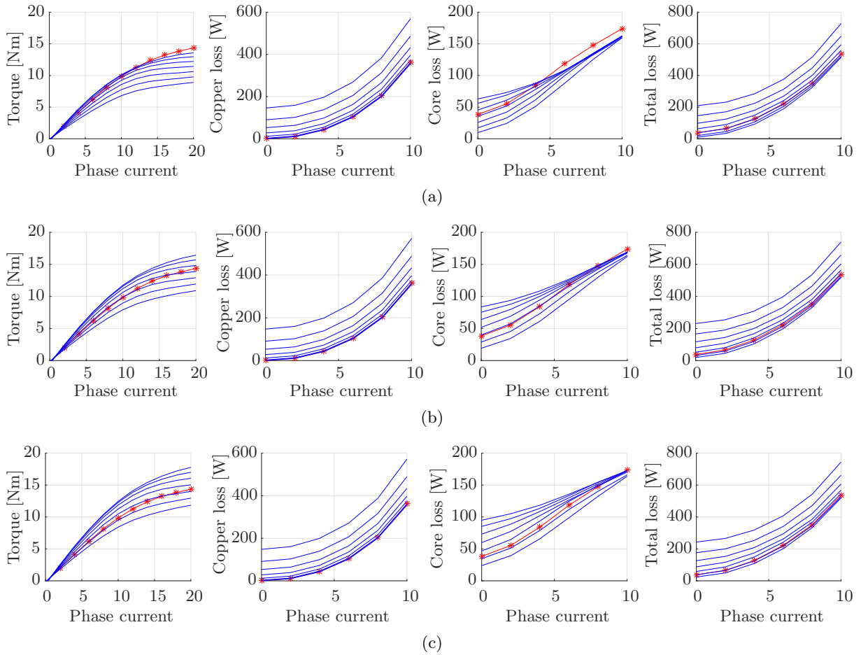
Fig. 5.17: Comparison between PMSM and DESM according to side PM thickness. Solid - DESM. Solid + star - PMSM. For DESM, I_{dc} = 0 \div 6A from bottom to top curves: a) 2 mm. b) 4 mm. c) 6 mm
