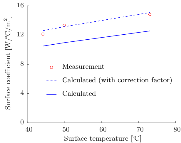
Fig. 4.22: Surface coefficient according to surface temperature at 20^\circ\text{C} ambient temperature
