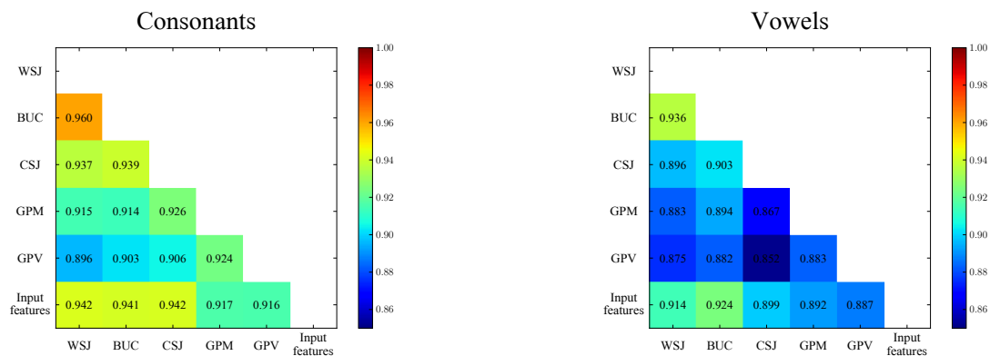
(a) For each pair of models: average over the different corpora of the correlation between the normalized ABX error rates for each pair of consonants.
