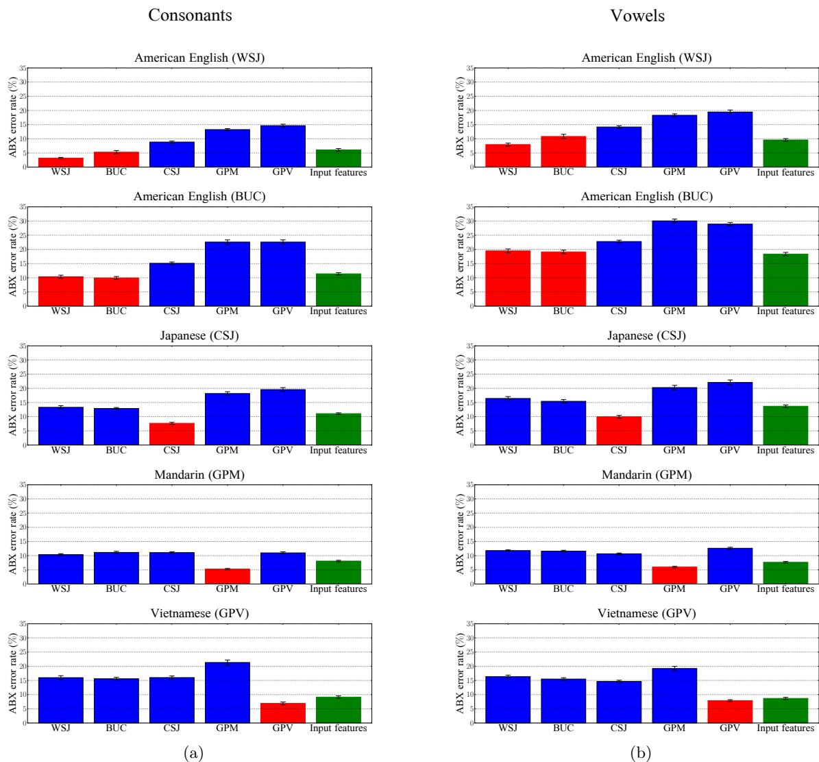
Figure 4.1: (a) Average ABX-discriminability of consonant contrasts. Columns correspond to the corpora on which the models were trained and lines correspond to the corpora on which they were tested. Red bars are used for the matching language conditions, i.e. where a model was tested on a corpus in the same language as the corpus on which it was trained. Blue bars are used for the mismatched language conditions, where a model was tested on a corpus in a different language than the corpus on which it was trained. Green bars are used for the baseline obtained by using as a representation the input features (MFCC plus pitch features) common to all models. Error bars indicates mean plus and minus one standard deviation and were obtained by bootstrap resampling of the scores at the level of the speakers. (b) As in (a), but for vowel contrasts.
