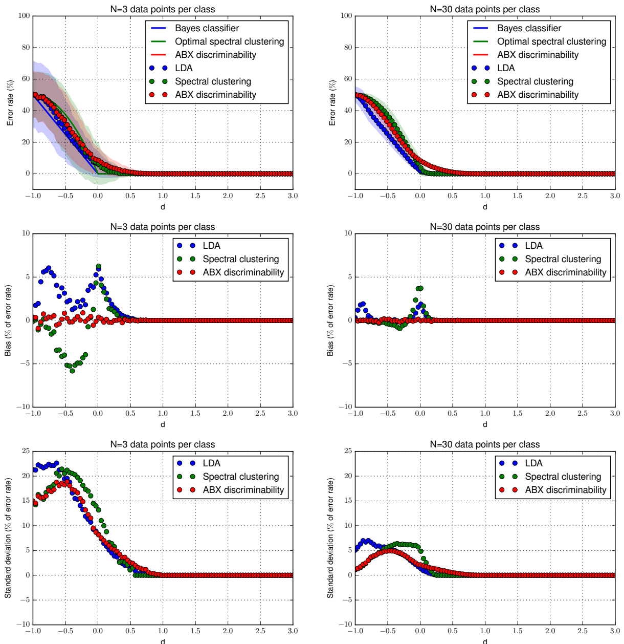
Figure 1.8: Comparison of the statistical efficiency of Linear Discriminant Analysis (LDA), spectral clustering and ABX-discriminability in the line example. Results for balanced samples with 3 data points per class are reported on the left panels, results for 30 data points per class in the right panels. Top panels contain the asymptotic error rates as a function of d for each method (straight lines), the average value of the finite sample estimates for each method (dots) and shaded confidence regions indicating the average of the finite samples estimates plus and minus their standard deviation. Middle panels contain the observed bias of the finite sample estimates as a function of d for each method. Bottom panels contain the observed standard deviation of the finite sample estimates as a function of d for each method.
