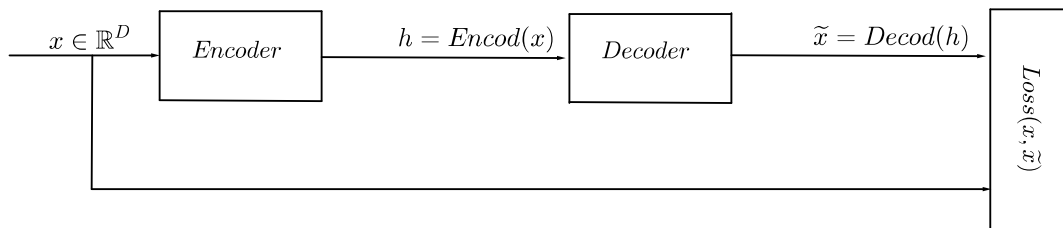
FIGURE 5.3: General Auto-Encoder structure.
