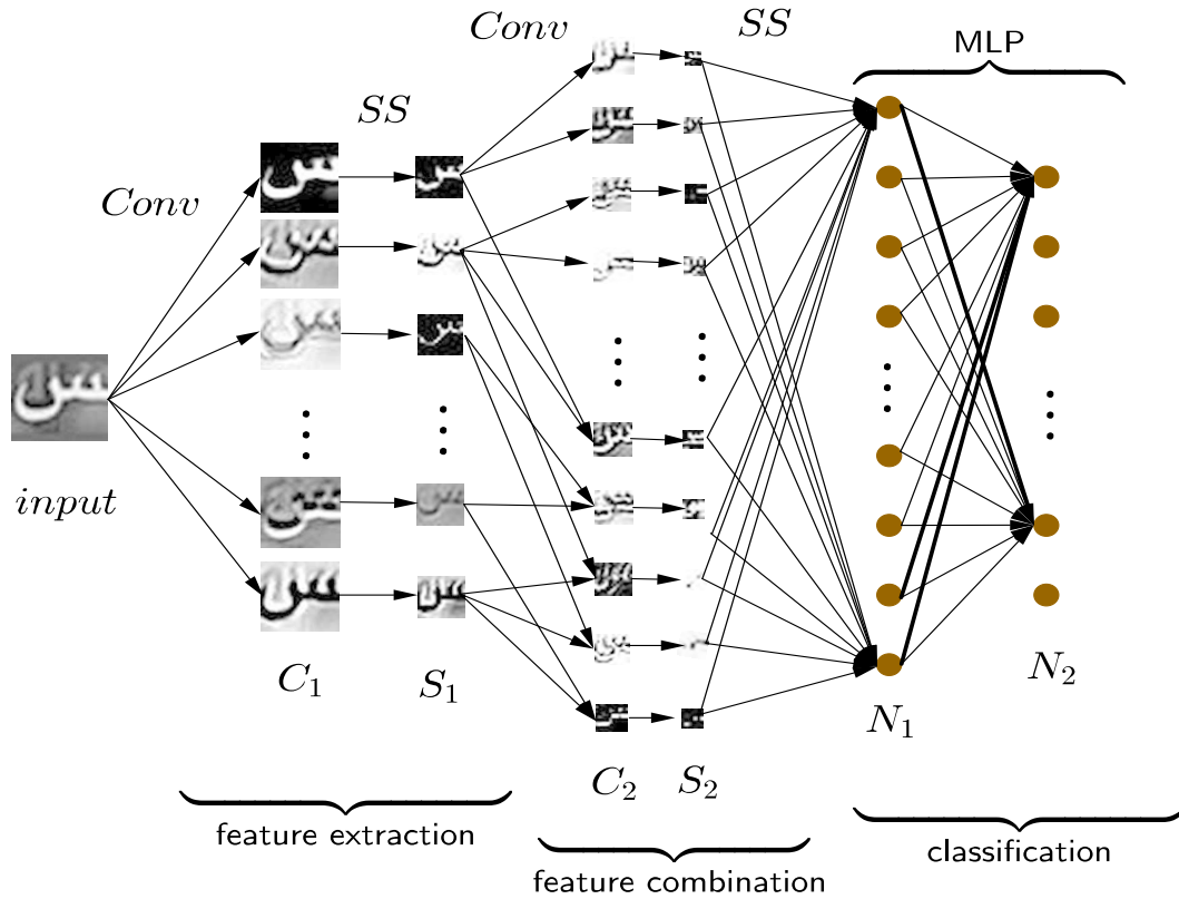
FIGURE 5.7: ConvNet-based character classifier. ‘Conv’ and ‘SS’ refer to convolution and sub-sampling operations respectively.
