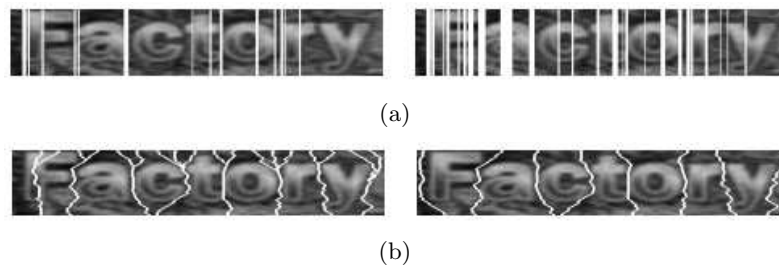
FIGURE 2.9: Character segmentation with both profile projection analysis (a) and the method based on gradient vector flow proposed in [PSST11] (b). (a) illustrates missed segmentation (left) and over-segmentation (right). (b) presents the forward pass (left) and backward pass (right) results of the proposed path finding method.
