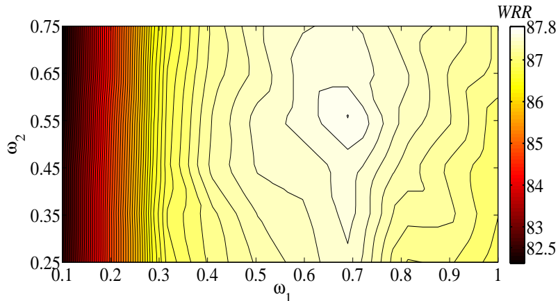
FIGURE 6.6: Recognition results variation with respect to LM weights.
