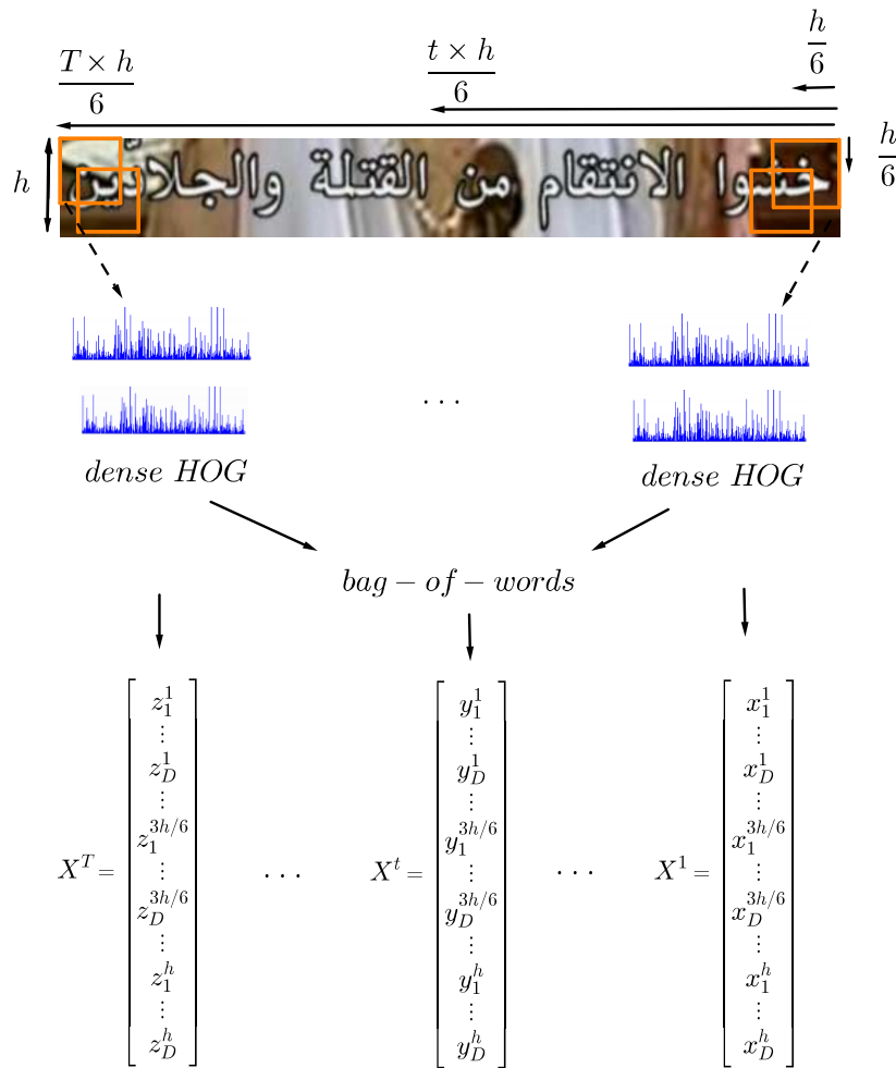
FIGURE 5.17: HOG-based text feature extraction.
