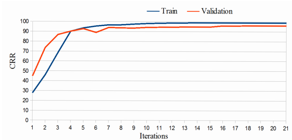
FIGURE 5.20: Evolution of training without the extra font.
