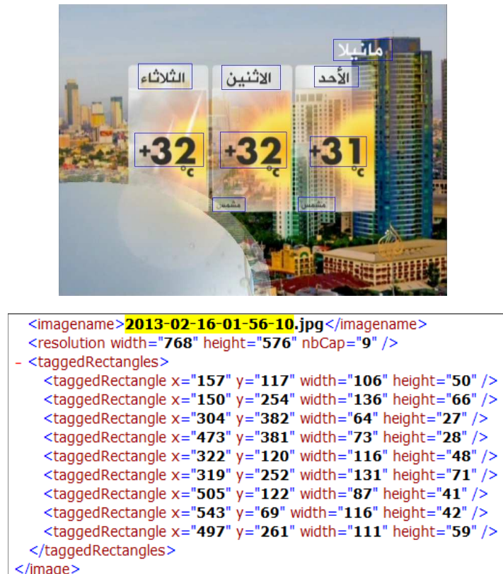
FIGURE 3.4: Example of detection-based annotation.
