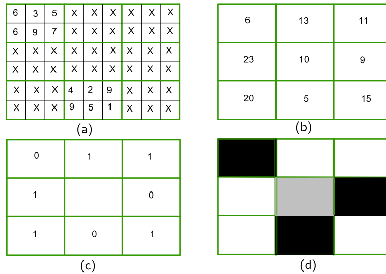
FIGURE 4.2: MBLBP: (a) region of an image divided into rectangles, (b) the average values of rectangles are calculated, (c) comparing central rectangle value with its neighborhood rectangles to provide a binary sequence defining in (d) the MBLBP relative to this region.
