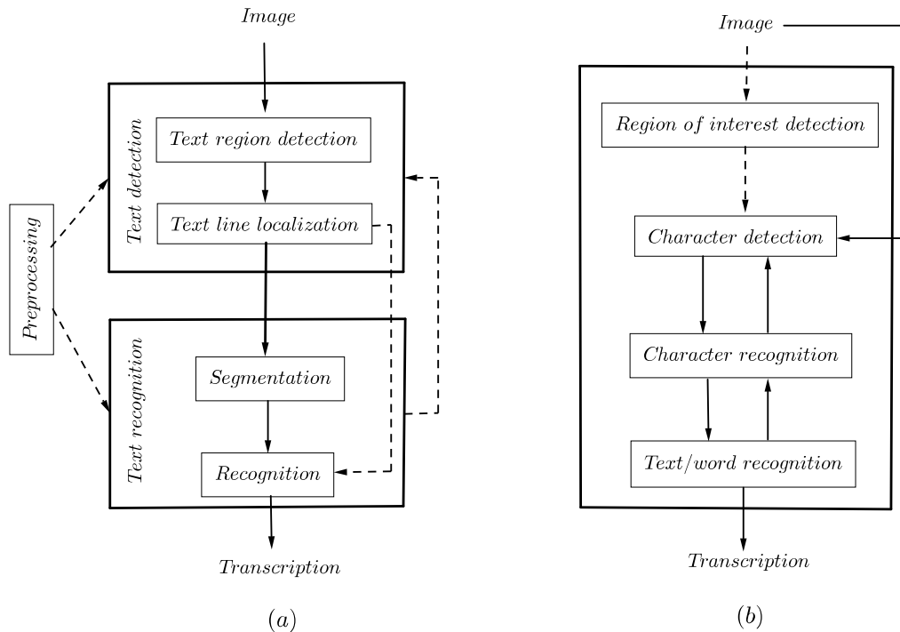
FIGURE 2.1: Text detection and recognition methodologies: (a) stepwise schema and (b) integrated schema.
