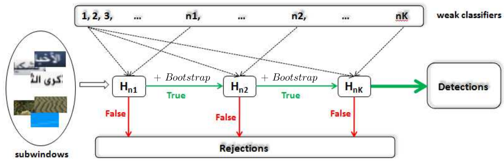
FIGURE 4.3: Multi-exit boosting cascade structure
