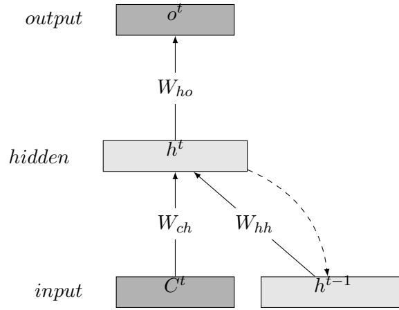
FIGURE 6.1: RNN-based LM architecture
