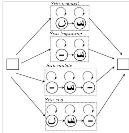
FIGURE 2.7: HMM structure for Arabic character ‘Siin’ using the sub-character model proposed in [ARFM13].
