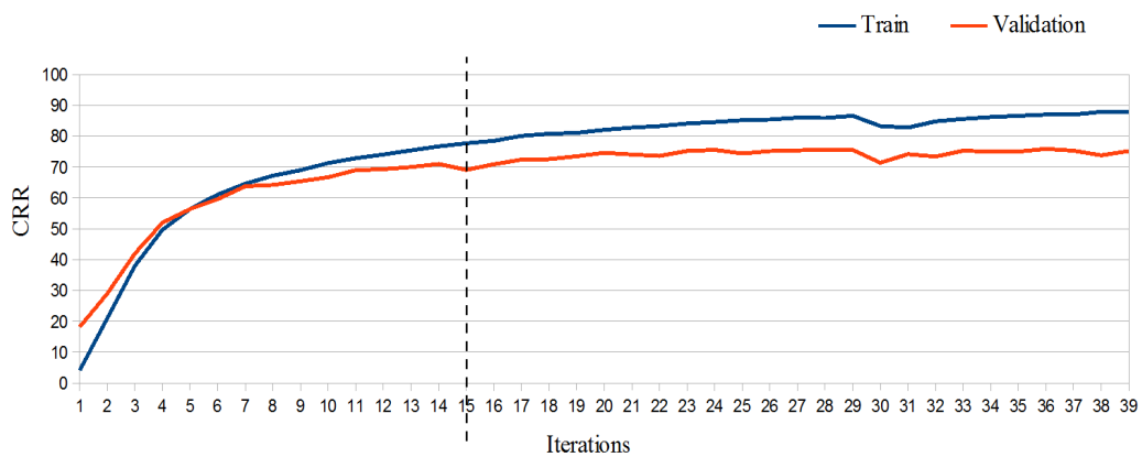
FIGURE 5.19: Evolution of initial training (the considered extra font is included in training set).
