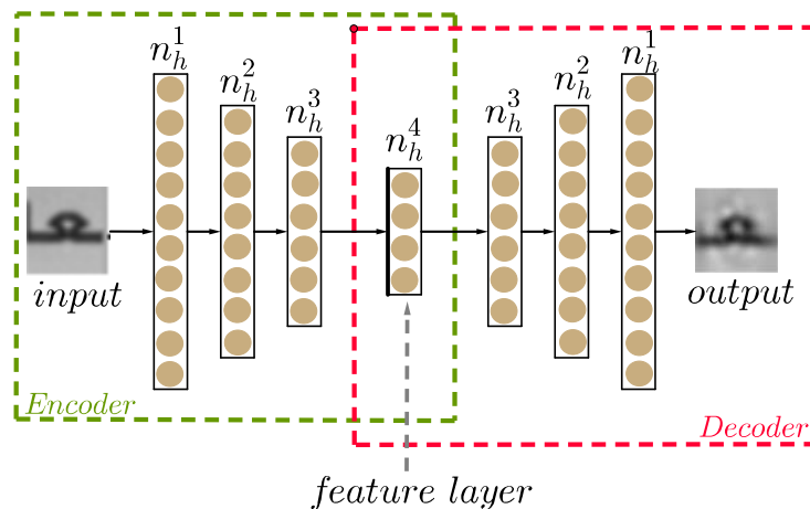
FIGURE 5.5: Deep Auto-Encoder formed by ‘unrolled’ RBMs.
