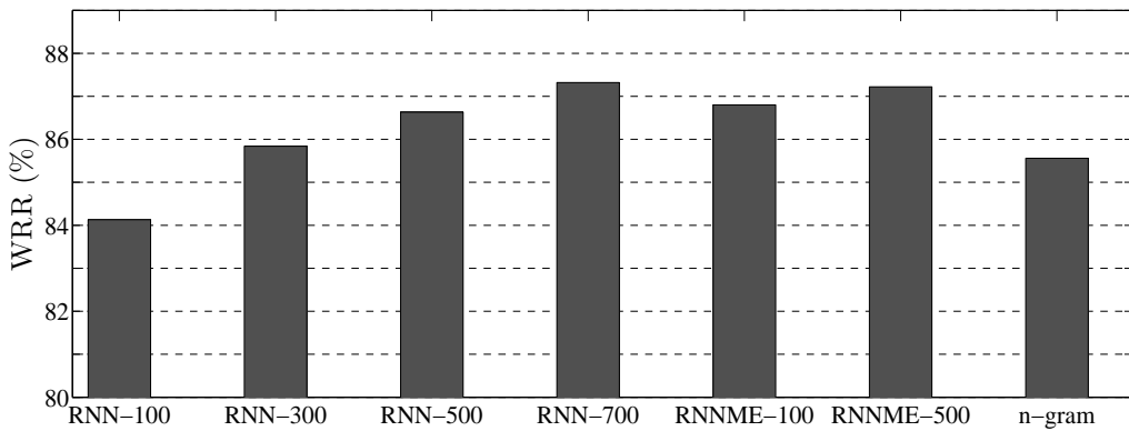
FIGURE 6.4: Primary impact of the proposed LMs integration on the text recognition results - Evaluation on the DEV_Set text images.
