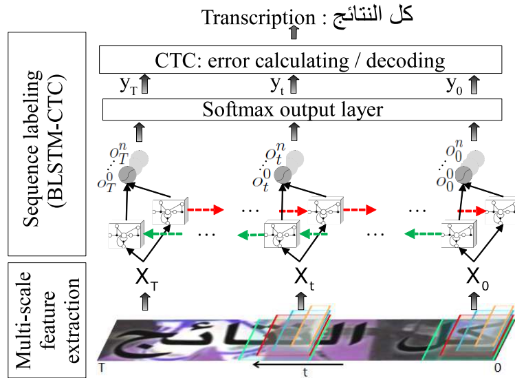
FIGURE 5.1: General overview of the proposed approach.
