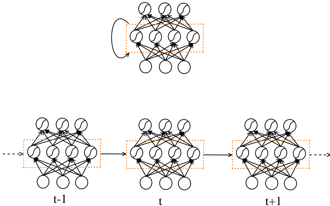
FIGURE 5.9: Architecture of a simple RNN with one hidden layer. Both compact (top) and unfolded in time (bottom) views are presented.
