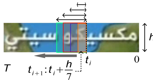
FIGURE 5.2: Multi-scale scanning procedure.
