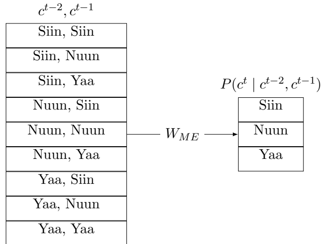
FIGURE 6.2: Maximum Entropy model with 3-gram features.
