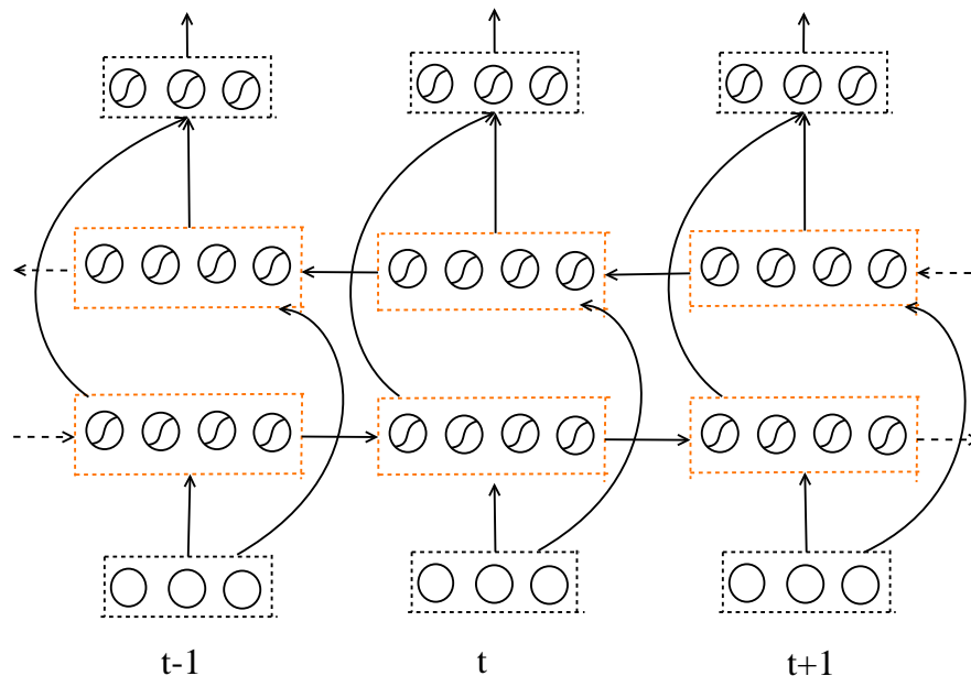
FIGURE 5.10: Architecture of a simple Bidirectional RNN.
