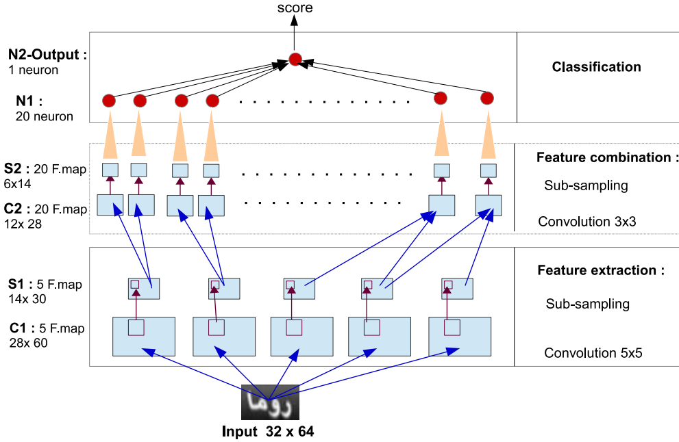
FIGURE 4.1: Convolution Neural Network architecture.
