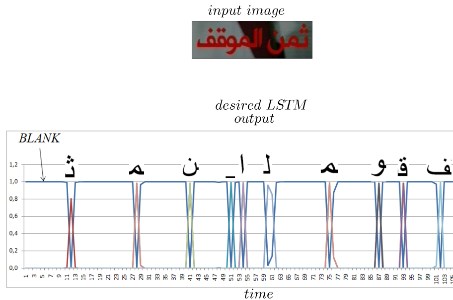
FIGURE 5.12: LSTM/RNN target output units activation through time. Curves represent the activation level through time of a set of label classes (label probability). ‘.’ corresponds to the space character. Most of times the network emissions correspond to the ‘BLANK’ class.
