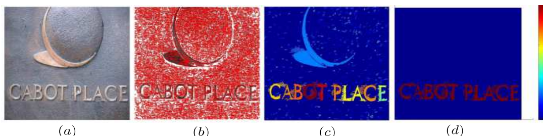
FIGURE 2.5: Text detection method used in [HQT14]. (a) Original image, (b) MSER component candidates, (c) component confidence map after applying ConvNet and (d) final detection after a simple thresholding.
