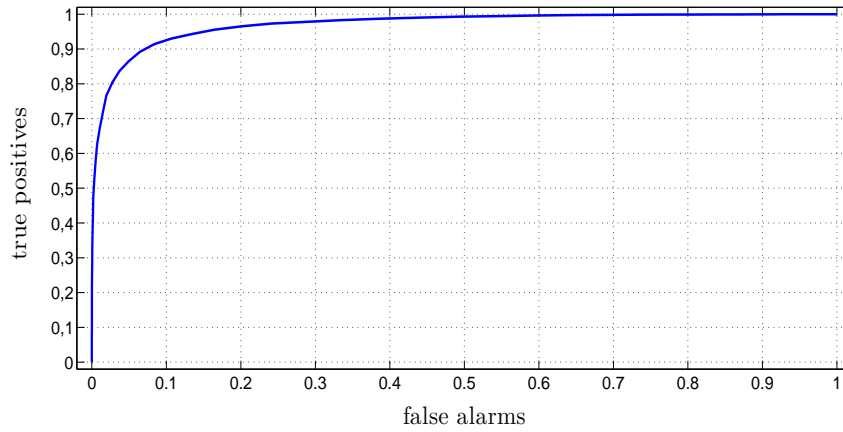
(a) MBLBPgentle.
