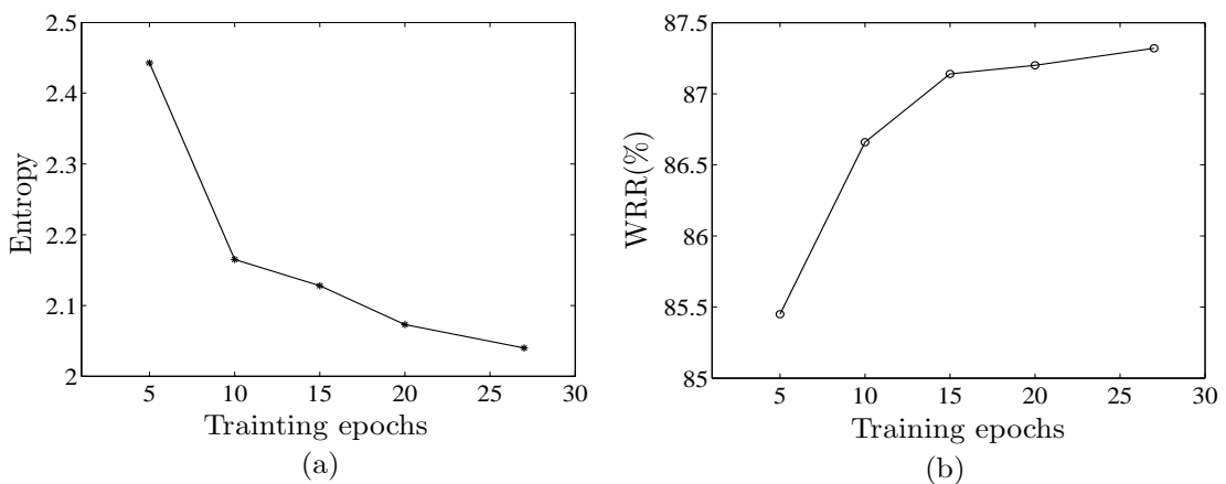
FIGURE 6.5: Evolution of the RNN-700 LM results during training: (a) progressive reduction in the entropy per character on the TEXT_Test set. (b) a corresponding improvement in WRR after joint decoding applied to the DEV_Set text images, using the RNN-700 configuration after each training epoch.
