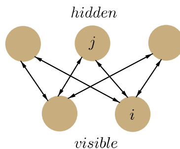
FIGURE 5.4: Diagram of Restricted Boltzmann Machine with 2 visible units and 3 hidden units.
