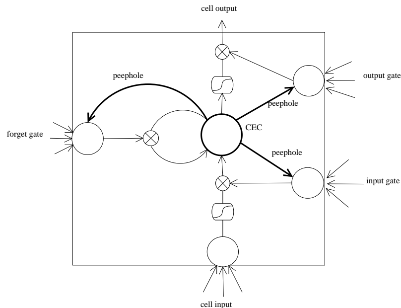
FIGURE 5.11: Graphical representation of a LSTM memory block with one cell.
