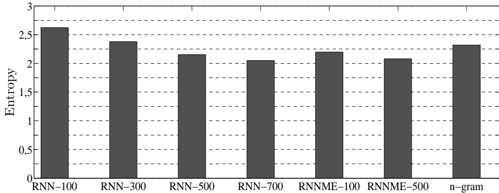
FIGURE 6.3: Evaluation of the proposed LMs in terms of entropy on the TEXT_Test set.
