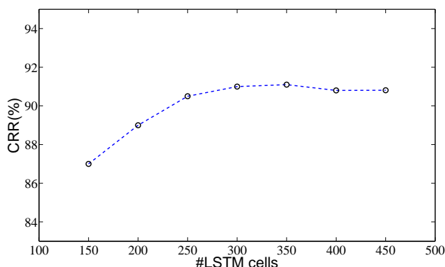
FIGURE 5.16: Impact of the number of LSTM cells.
