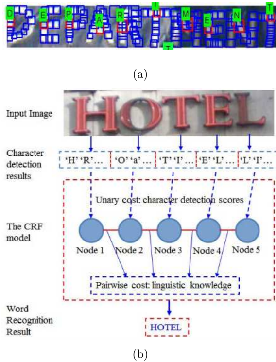
FIGURE 2.11: Illustration of the proposed word recognition method in [SWX + 13]. (a) presents an example of the character recognition and detection using tree-structured models. (b) summarizes the whole used word recognition paradigm.
