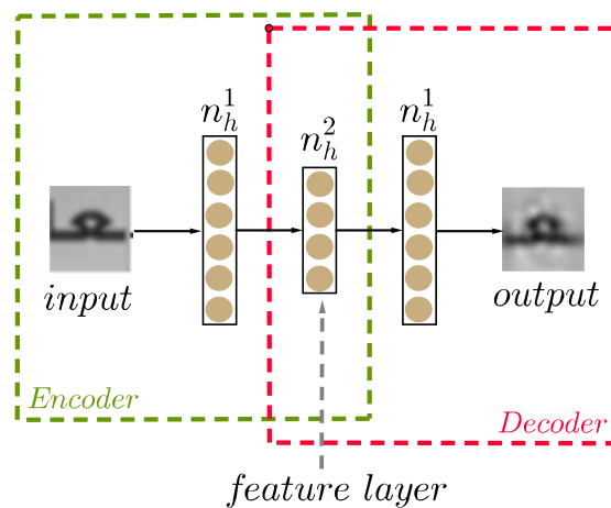
FIGURE 5.6: MLP-based Auto-Encoder.
