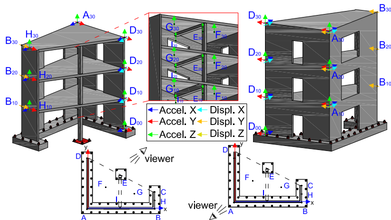
Figure 3.51: Measurement points.
