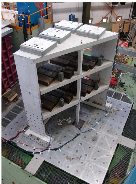
Figure 3.45: Picture of ENISTAT mock-up.
