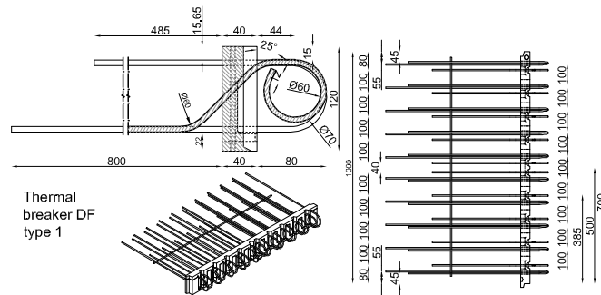
Figure 3.48: Drawing of the DF type 1 thermal break component.
