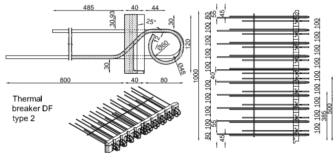
Figure 3.49: Drawing of the DF type 2 thermal break component.
