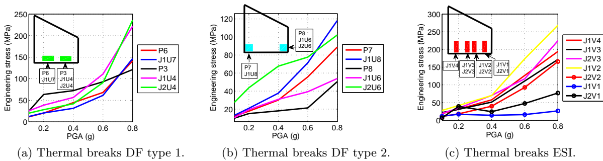
Figure 3.58: Maximum engineering stress versus seismic ground motion level — shear wall #2.
