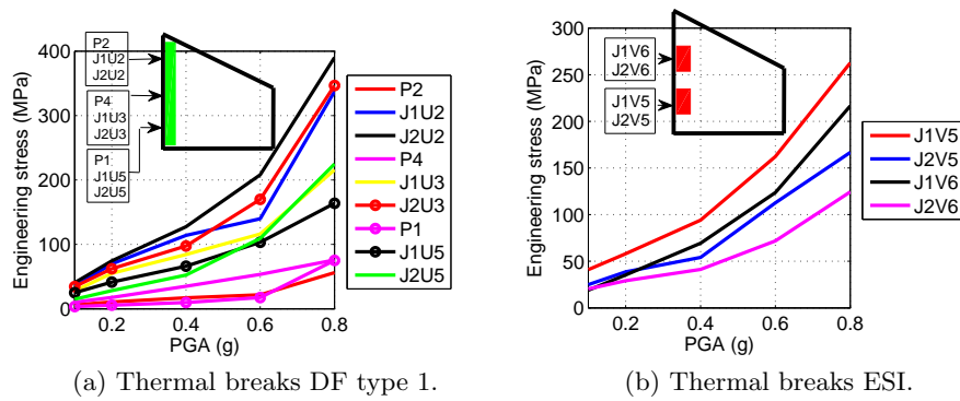
Figure 3.57: Maximum engineering stress versus seismic ground motion level — shear wall #1.
