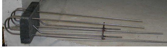
Figure 3.47: Picture of a thermal break component.
