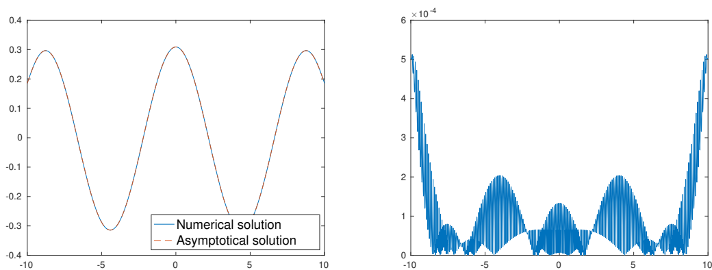
Figure 2.4.11: Comparison of asymptotical and numerical values for n = 5 eigenfunction (3rd even eigenfunction), \beta = 0.1 : eigenfunction values (left) and difference between asymptotical and numerical solutions (right)
