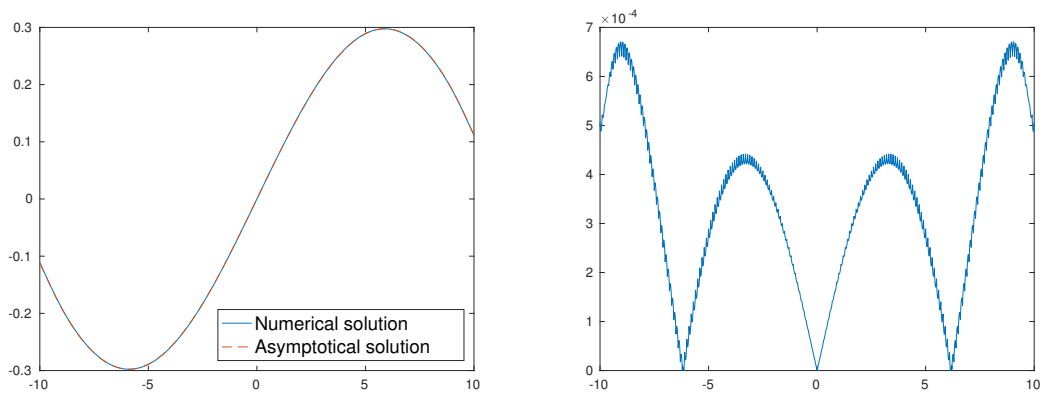
Figure 2.4.14: Comparison of asymptotical and numerical values for n = 2 eigenfunction (1st odd eigenfunction), \beta = 0.1 : eigenfunction values (left) and difference between asymptotical and numerical solutions (right)
