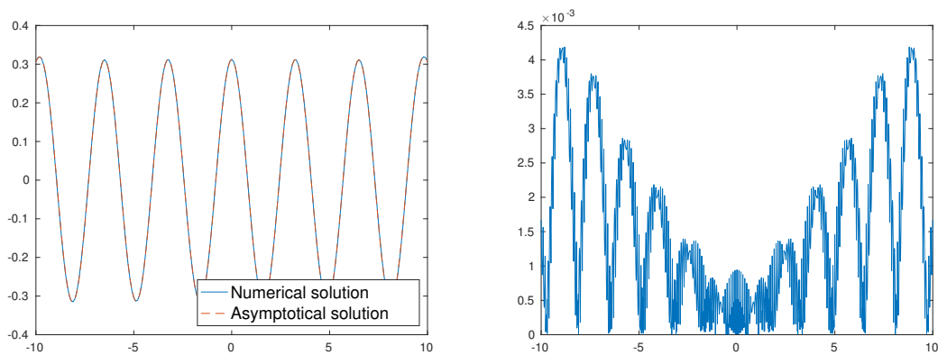
Figure 2.4.12: Comparison of asymptotical and numerical values for n = 13 eigenfunction (7th even eigenfunction), \beta = 0.1 : eigenfunction values (left) and difference between asymptotical and numerical solutions (right)
