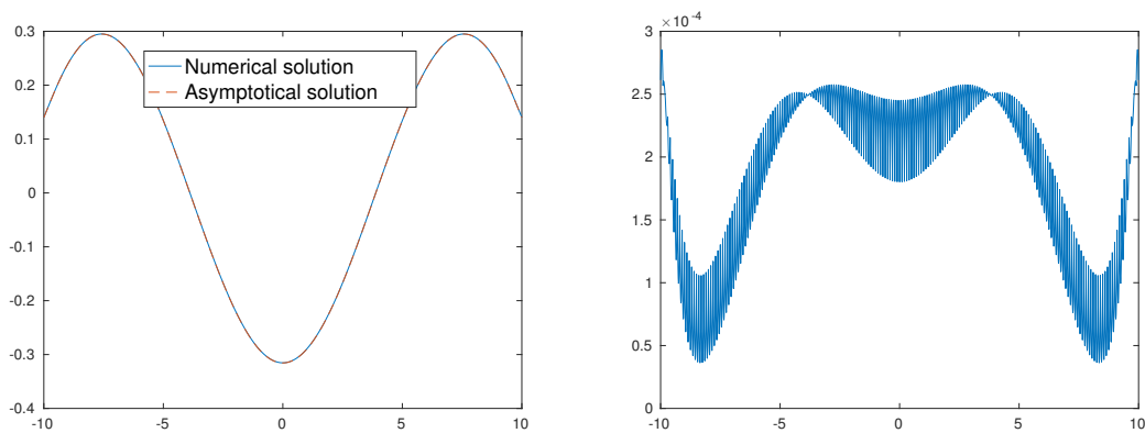
Figure 2.4.10: Comparison of asymptotical and numerical values for n = 3 eigenfunction (2nd even eigenfunction), \beta = 0.1 : eigenfunction values (left) and difference between asymptotical and numerical solutions (right)
