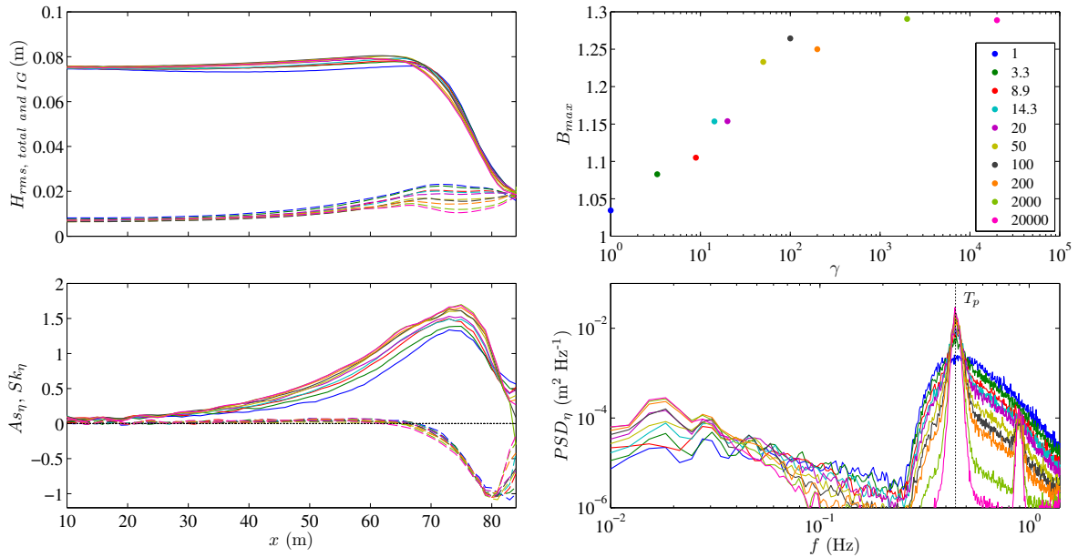
Figure 3.33: Influence of offshore \gamma on H_{rms} (solid line - total; dashed line - IG waves only), S_k (solid line) and A_s (dashed line) and B_{max} . The last plot shows the spectra of free-surface elevation at the first wave gauge. Note: the purple curves correspond to A3T run.
