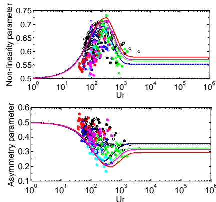
Figure 5. Dibajnia et al. (2001) parameterization for nonlinearity and asymmetry parameters (lines) and field data (symbols), considering T_z instead of T_s , for calculation of the Ursell number (defined according to equation 3).
