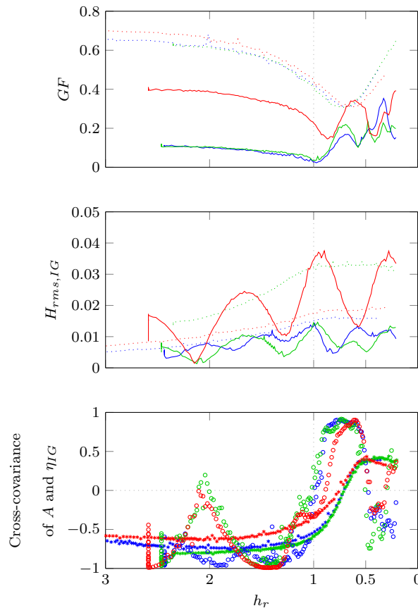
Figure 3.11: Top: Groupiness factor along the beach profile. Cross-shore positions corresponding to h_r < 0.2 are excluded from analysis due to the known inaccuracy of the method for very-shallow water depths (List, 1991). Middle: IG-wave height. Bottom: Cross-covariance between the amplitude of the wave envelope and the IG-wave signal. For both A (dotted lines or asterisks) and B (solid lines or circles) series, the blue, green and red colours represent conditions 1, 2 and 3, respectively. The dotted vertical grey lines mark the location of the breakpoint.
