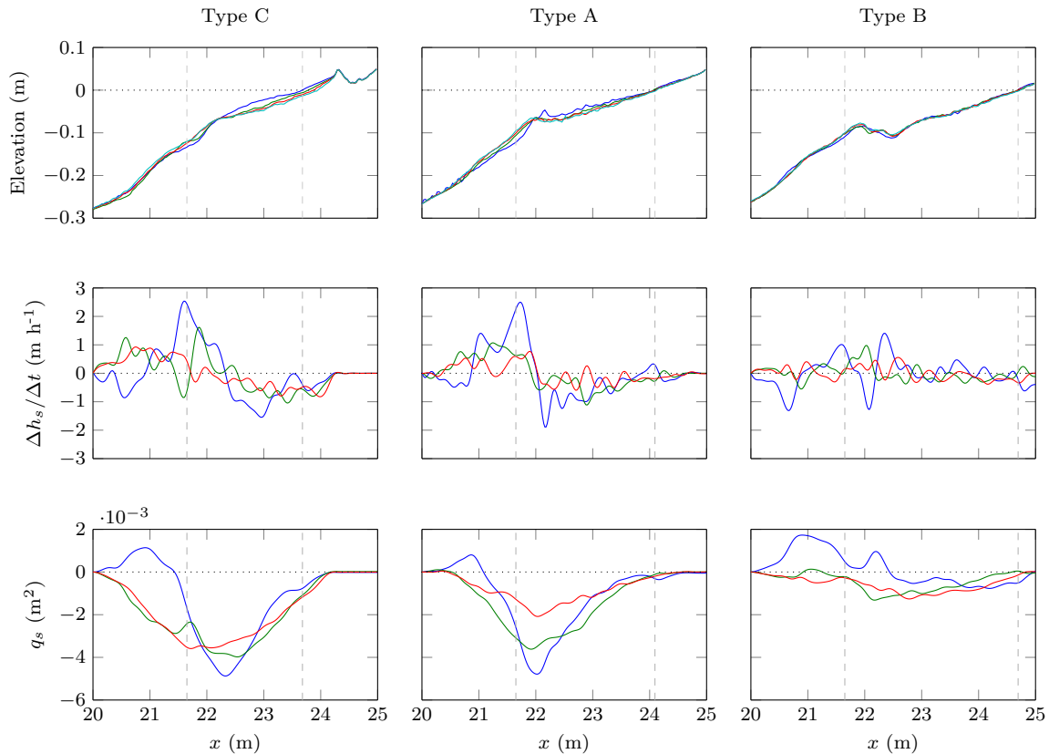
Figure 4.29: Beach profiles, variation of sediment height and bulk sediment transport for groups of three C2 short runs over initial beach profiles of types C, A and B. Color code, from the initial profile to the last one: blue, green, red and cyan (cyan for top plots only). Grey dashed lines mark the approximate position of the breakpoint and the shoreline.
