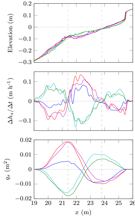
Figure 4.24: Beach profiles, variation of sediment height and bulk sediment transport for five C1 20-min runs. Color code, from the initial profile to the last one: blue, green, red, cyan, violet, yellow (yellow for the top plot only). Grey dashed lines mark the approximate cross-shore positions for which the bed remains at the same position during the five runs (nodal points of the bed-profile oscillation).
