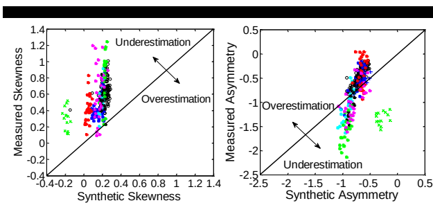
Figure 6. Measured skewness and asymmetry versus synthetic skewness and asymmetry computed following the method of Elfrink et al. (2006).
