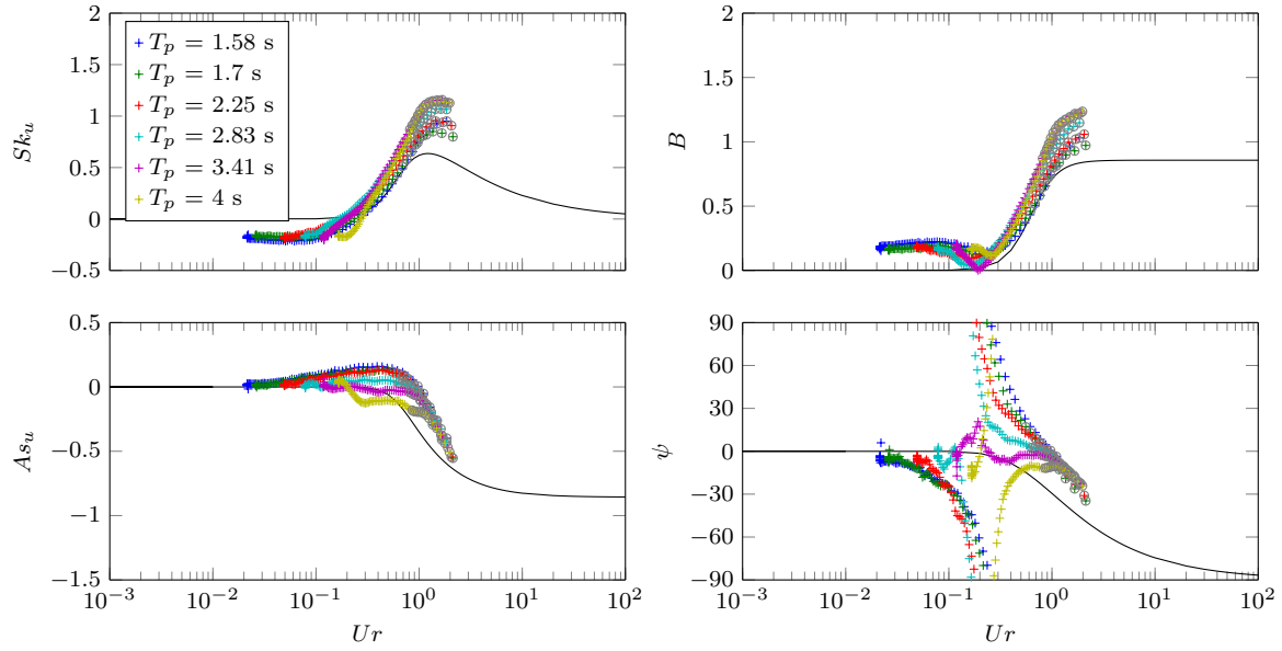
Figure 3.40: Velocity skewness, velocity asymmetry, B and \psi in function of U_r , for different- T_p runs. The black curves correspond to the RRR12 parameterization. Grey circles mark the data points corresponding to cross-shore positions after the breakpoint.
