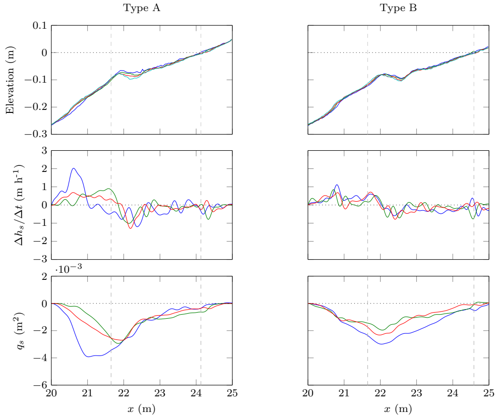
Figure 4.30: Beach profiles, variation of sediment height and bulk sediment transport for groups of three C1 short runs run over initial beach profiles of types A and B). Color code, from the initial profile to the last one: blue, green, red, cyan (cyan for top plots only). The grey dashed lines mark the approximate positions of the breakpoint and the shoreline.
