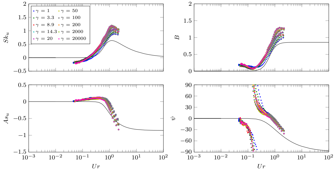
Figure 3.41: Velocity skewness, velocity asymmetry, B and \psi in function of the U_r , for different- \gamma runs. The black curves correspond to the RRR12 parameterization. Grey circles mark the data points corresponding to cross-shore positions after the breakpoint.
