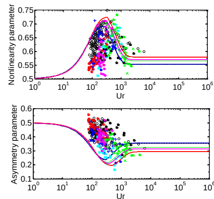
Figure 4. Dibajnia et al. (2001) parameterization for nonlinearity and asymmetry parameters (lines) and field data (symbols). Ur is defined according to (3).
