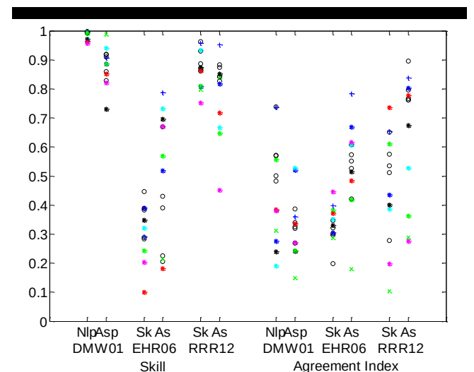
Figure 8. Skill and agreement index values calculated for skewness and asymmetry for each of the three parameterizations considered. Skewness skill value for EHR06, for Mira data set, is not presented in the plot for convenience ( \approx -0.5 ).
