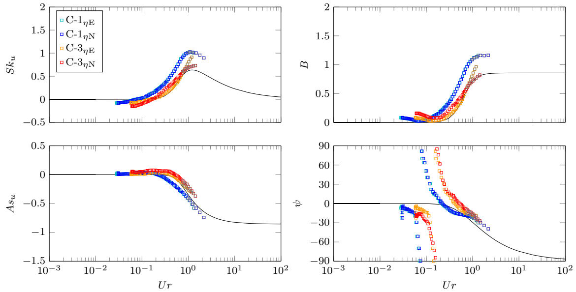
Figure 3.38: Velocity skewness, velocity asymmetry, B and \psi in function of Ur , for experimental ( u_\eta from \eta_E )/numerical ( u_\eta from \eta_N ) velocity time series C-1 (cyan/blue) and C-3 (orange/red). The black curves correspond to the RRR12 parameterization. Grey circles mark the data points corresponding to positions after the breakpoint.
