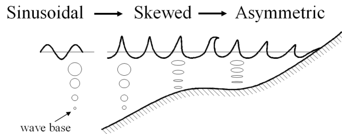
Figure 2.5: Sketch of the wave-shape transformation and corresponding orbital motions as waves propagate from deep to shallow waters (Abreu, 2011).
