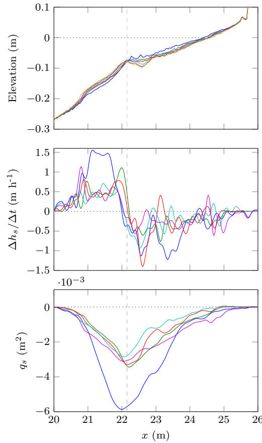
Figure 4.41: Beach profiles, variation of sediment height and bulk sediment transport for five C1 short runs. Color code, from the initial profile to the last one: blue, green, red, cyan, violet, yellow (yellow for the top plot only). The grey dashed lines mark the approximate position of the breakpoint.
