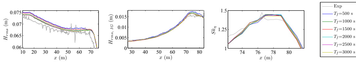
Figure 3.20: Sensitivity of the wave statistics to the length of the runs (A1 example). Spatial distribution of H_{rms} , H_{rms,IG} and Sk_\eta in the zones of the cross-shore profile where these variables show a greater variation depending on the run length.
