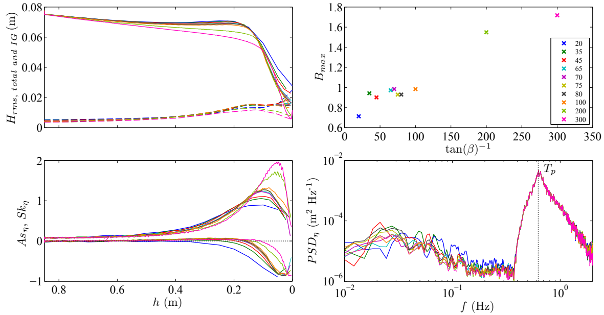
Figure 3.34: Influence of \tan(\beta) on H_{rms} (solid line - total; dashed line - IG waves only), Sk_\eta (solid line) and A_{s\eta} (dashed line) and B_{max} . The last plot shows the spectra of free-surface elevation the first wave gauge.
