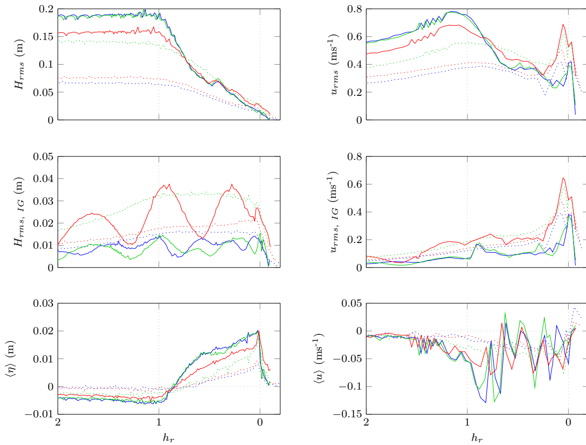
Figure 3.9: Cross-shore evolution of H_{rms} and u_{rms} for the total signal and IG-frequencies only, mean water level and mean velocity. For both A (dotted lines) and B (solid lines) series, the blue, green and red colours represent conditions 1, 2 and 3, respectively. The dotted vertical grey lines mark the location of the breakpoint and the shoreline.
