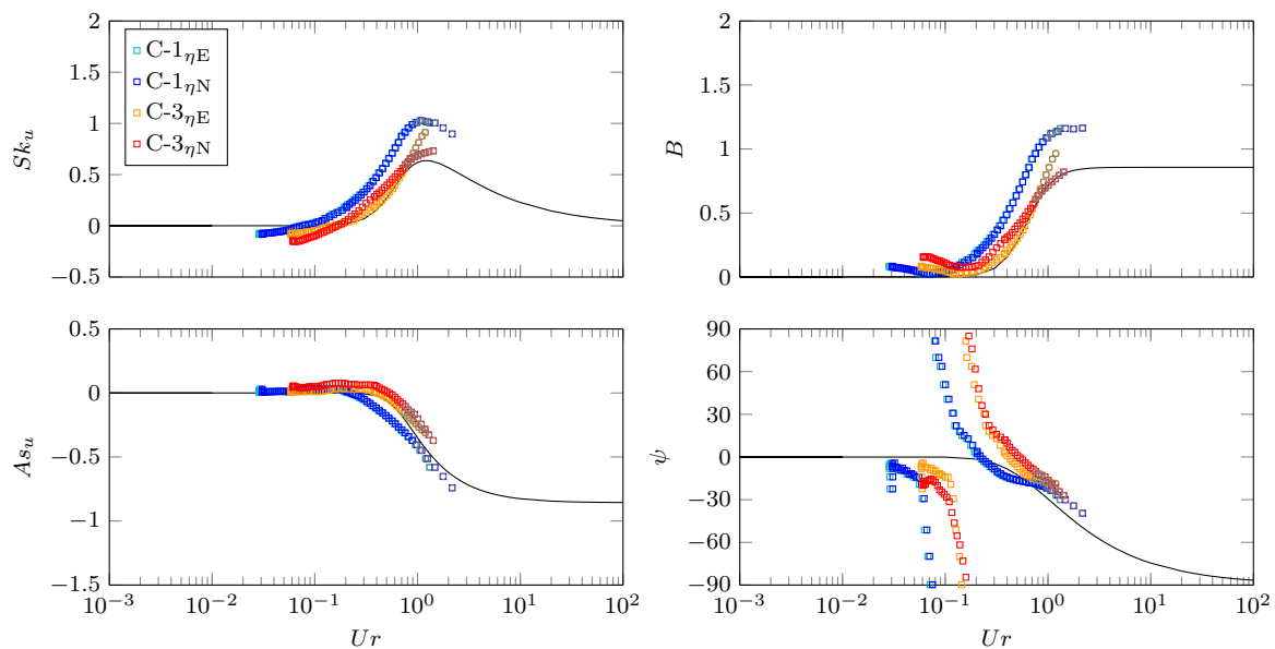
Figure 3.38: Velocity skewness, velocity asymmetry, B and \psi in function of U_r , for experimental ( u_\eta from \eta_E )/numerical ( u_\eta from \eta_N ) velocity time series C-1 (cyan/blue) and C-3 (orange/red). The black curves correspond to the RRR12 parameterization. Grey circles mark the data points corresponding to positions after the breakpoint.
