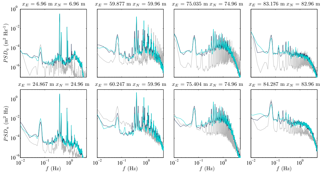
Figure A.5: Spectra of free-surface elevation (top) and cross-shore velocity (bottom) at four different cross-shore positions for B1 (with \phi_b = 27^\circ and \phi_f = 9^\circ ). Grey line - experimental data; dark blue - B1E; blue - B1T.
