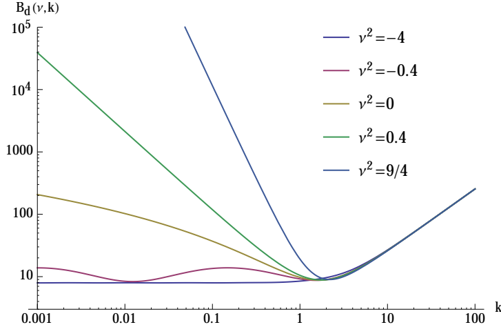
Figure 2.2: The function B_d(\nu, k) [see Eq. (2.21)] in D = 3 + 1 dimensions versus k for various (real and imaginary) values of \nu . In the UV regime k \gtrsim 1 the function B_d(\nu, k) \sim k , which reproduces the Minkowski beta function for the potential. Imaginary values of \nu correspond to regions of field space where the curvature of the potential V_k'' > d^2/4 . In that case, the function B_d(\nu, k) shows a bounded oscillatory behavior for k \lesssim 1 and it is essentially constant for large field curvatures, V_k'' \gg d^2/4 . For \nu = 0 , this turns into a logarithmic behavior, which reflects the gravitational enhancement of superhorizon fluctuations. Finally, real positive values of \nu correspond to regions of field space where the curvature of the potential V_k'' < d^2/4 and are most sensitive to space-time curvature effects. The logarithmic enhancement is turned into a power law k^{-2\nu} .
