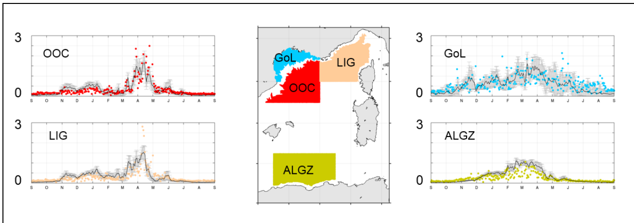
Figure 4: September 2012 to September 2013 Sea Surface Chlorophyll-a concentration [mg.m -3 ] comparison between model outputs (black line for the spatial average and grey regions for the standard deviation) and MODIS 4km resolution satellite products (the colours refer to the regions of the map).
