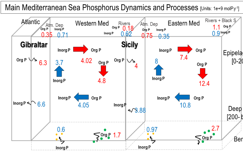
Figure 16: Mediterranean phosphorus cycle. Org represents the organic matter and Inorg represents the inorganic matter amount. Unit: 10^9 molP.y -1 .
