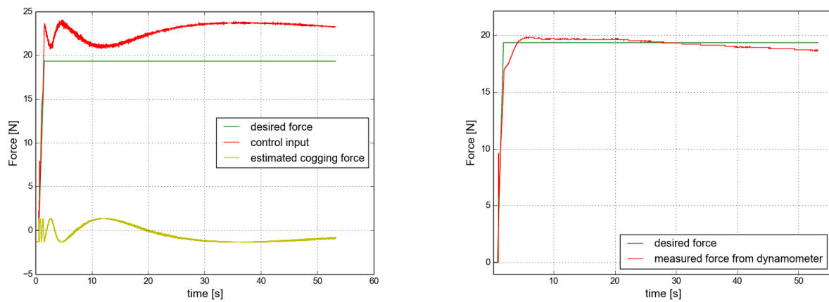
(a) Desired force, estimated cogging force and force given as input to the controller ( f_{cable}^* ) after torque feed-forward (obtained from current readings). (b) Comparison between the measured force and the desired one.
