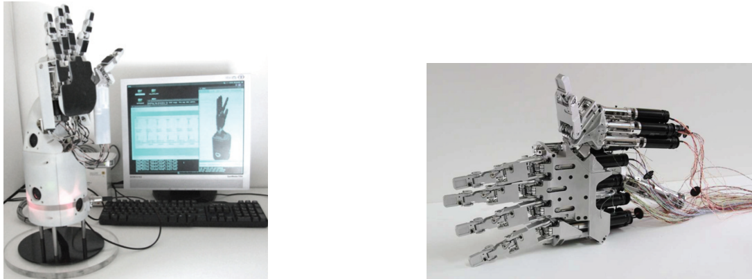
Figure 1.14 – The CEA dexterous hand. Pictures taken from [53].
