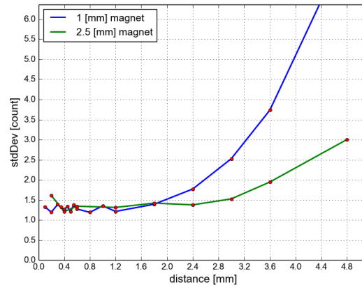
Figure D.2 – SD_x magnets comparison.
