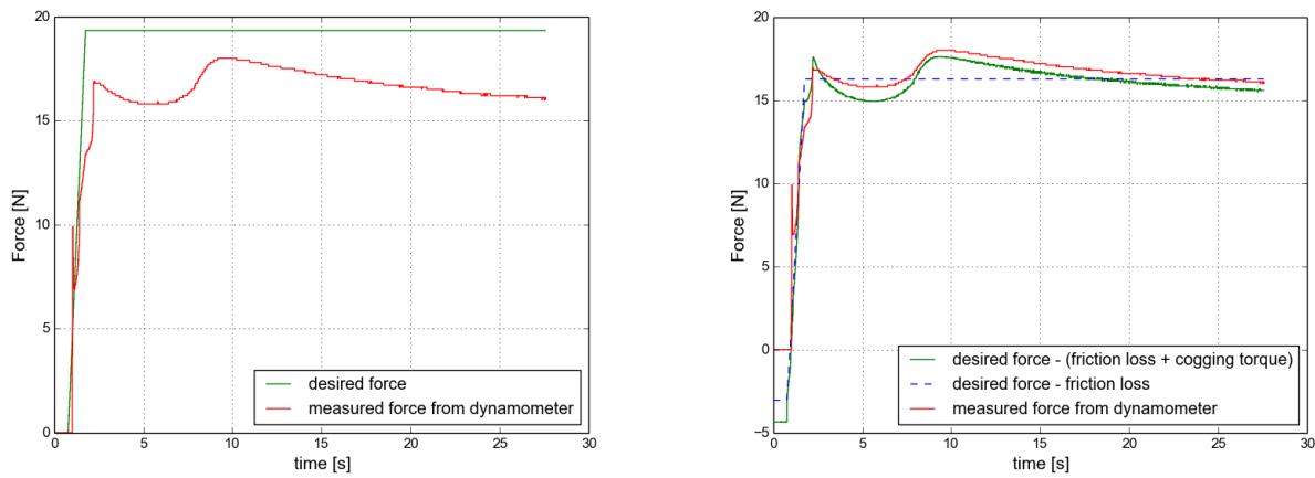
(a) Force control performance without torque feed-forward. (b) Identification of disturbance factors on the output pulling force.
