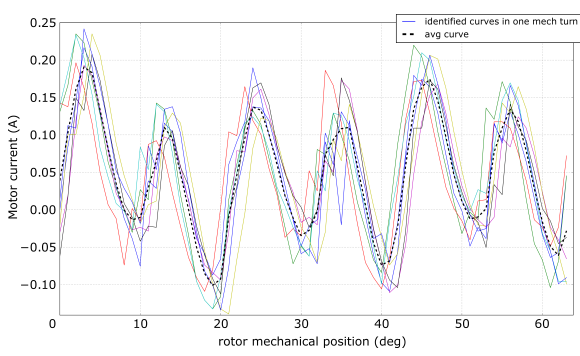
(a) Averaged motor currents on an electrical turn. Data are acquired in a complete mechanical turn.
