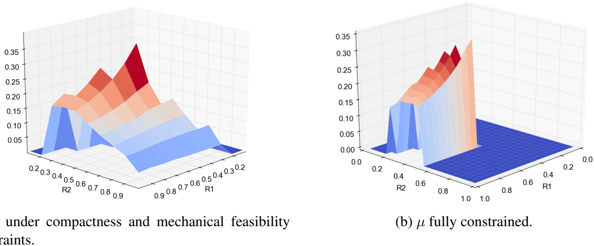
Figure 4.8 – Analysis of \mu under stability, compactness and mechanical feasibility constraints.
