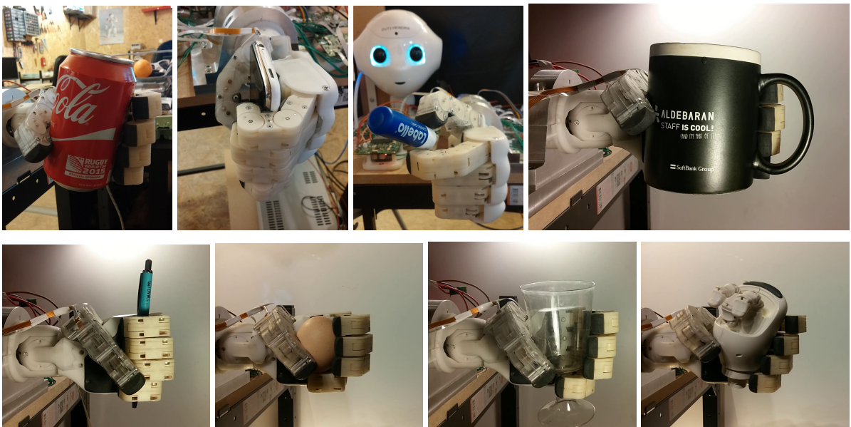
Figure 6.12 – Selection of small and light objects grasped by ALPHA.
