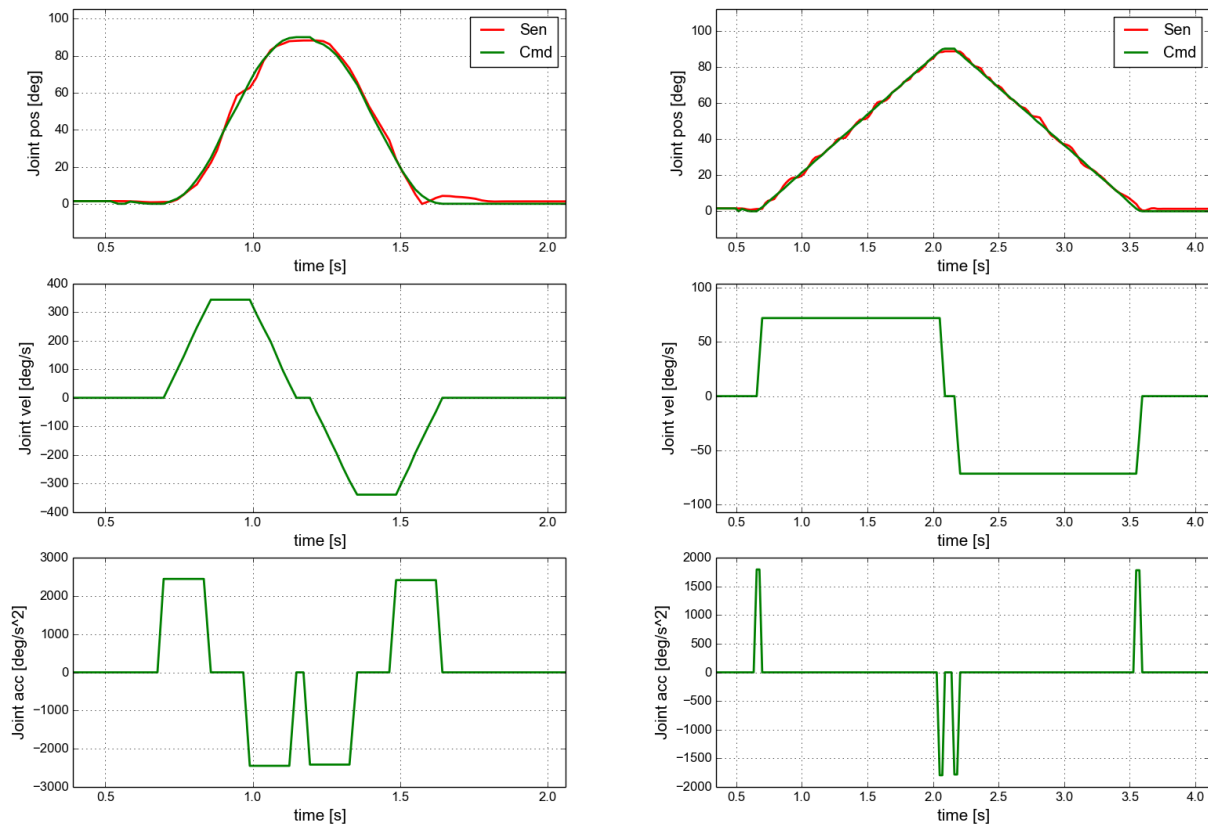
(a) Open/close finger motion under 1 [s].
