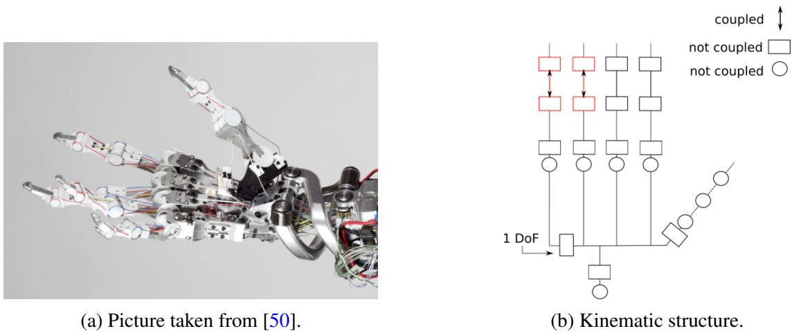
Figure 1.12 – The hand of the DLR Hand Arm System.
