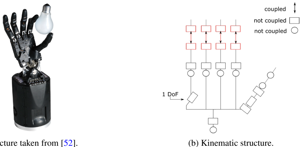
Figure 1.13 – The Shadow hand.
