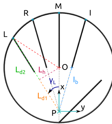
Figure 2.5 – Definition of finger base positions (palmar view).
