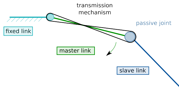
Figure 3.1 – Transmission mechanism terminology.
