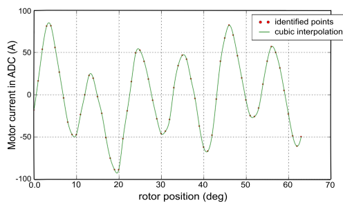
Figure 4.22 – Values i_q stored on the motor board and added to i_q^* to compensate cogging torque effects.
