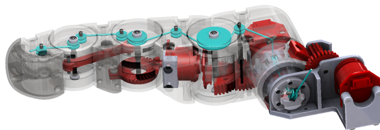
Figure 5.19 – ALPHA thumb design: parallel e-motion and grasp transmission mechanisms. The e-motion brushless DC motors, gears and elastic coupling bar are highlighted in red while the grasp cable and pulleys are presented in blue.
