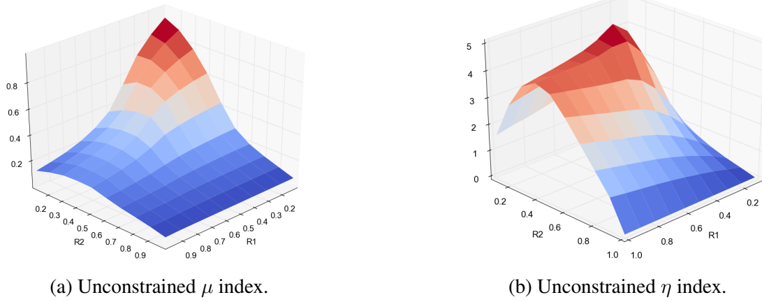
Figure 4.7 – Analysis of \mu and \eta indices in function of R_1 and R_2 over the full finger grasp state.
