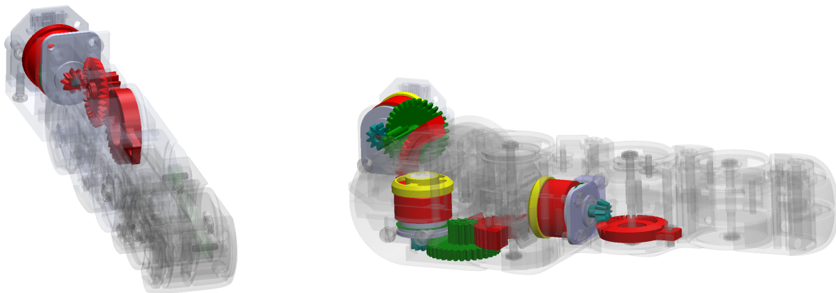
(a) Gear train for a generic finger.
