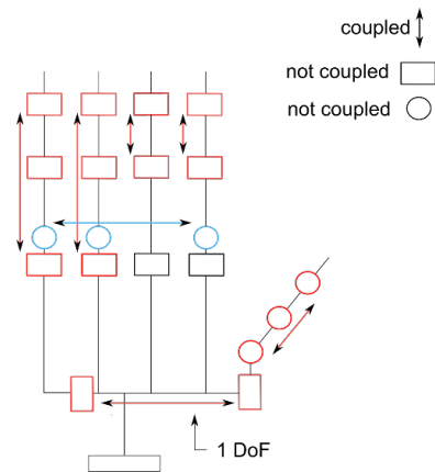
(b) Kinematic structure.
