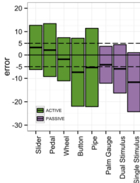
Fig. 1. Error (accuracy) and standard deviation (precision) according to the interaction technique. The palm gauge, the Pedal, the Slider and the wheel are significantly more accurate (smaller error) and more precise (smaller SD) than the other techniques. Dotted lines show +5 and -5 limits.
