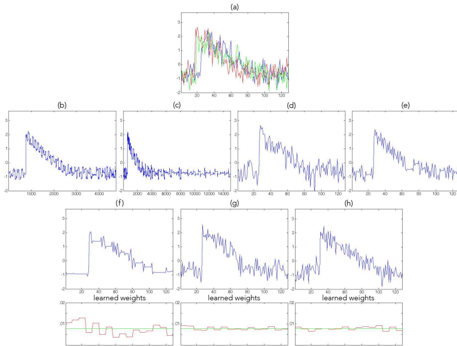
Figure 4.14: CBF-"Funnel" centroids: (a) Initial time series, (b) NLA AF, (c) PSA, (d) CWRT, (e) DBA, (f) WDTW, (g) WK_{DTAK} , (h) WK_{GDTW}
