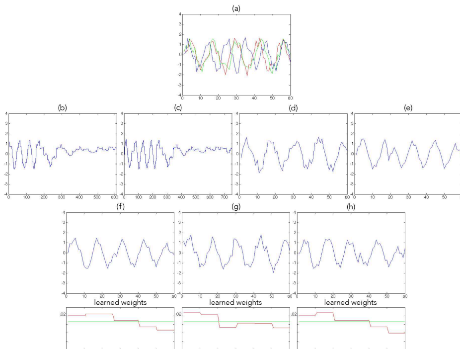
Figure 4.15: CC-"Cyclic" centroids: (a) Initial time series, (b) NLA AF, (c) PSA, (d) CWRT, (e) DBA, (f) WDTW, (g) WK_{DTAK} , (h) WK_{GDTW}
