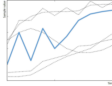
Figure 2.3: Medoid as a prototype
