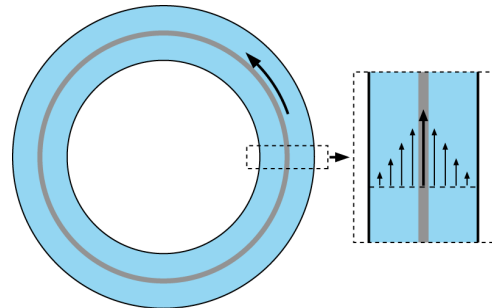
(b) Top view of the interface sheared by the rotation of the ring (grey). A torque (stress) is applied and the rotation (deformation) is measured.
