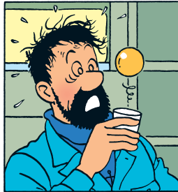
Figure 1.8: In microgravity, the shape of the liquid phase (here, the whiskey) is set to minimize its area with air, which leads to a sphere. (©Hergé/Moulinsart 2016)
