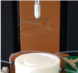
(a) Interfacial rheometer with "Double-wall ring" geometry. Ring and rheometer are provided by TA Instruments.
