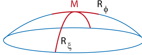
Figure 1.9: The pressure difference between both sides of the interface is defined by interfacial tension and the two radii of curvature of the surface.
