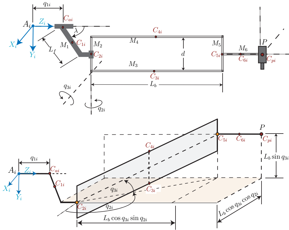
Figure 4.6 – Orthoglide 3-axis i^{\text{th}} leg
