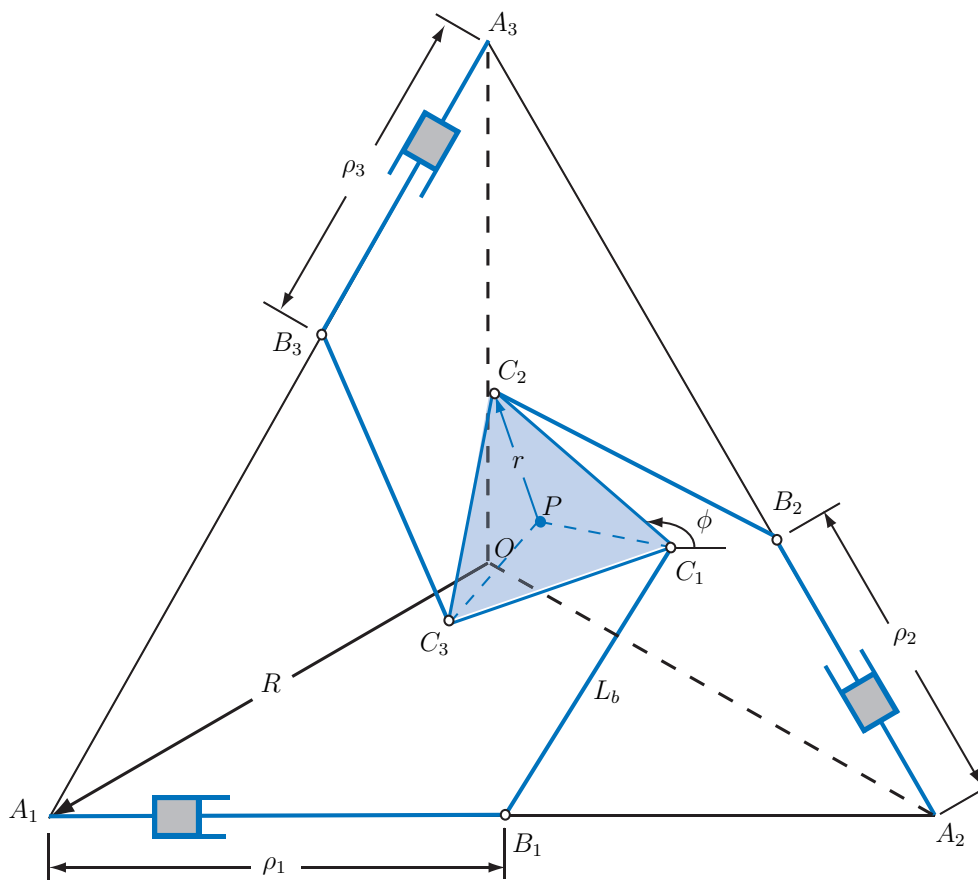
Figure 2.2 – 3- PRR architecture
