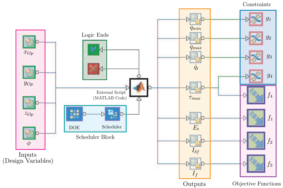
Figure 4.18 – modeFRONTIER model
