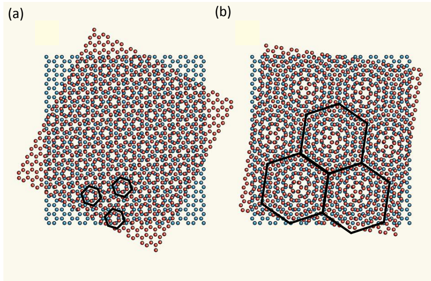
FIGURE 2.16: (a) The two lattices are overlaid at an angle of about 27.8^\circ . The resulting atomic arrangement is precisely periodic. (b) Lattices rotated by 9^\circ . Although the atomic arrangement never precisely repeats, there is a periodic pattern of points in space at which atoms from the two layers are nearly on top of each other, making the structure appear more open in this top view [120].
