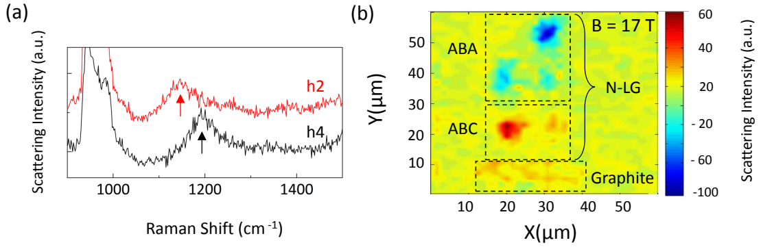
FIGURE 5.13: (a) Raman spectra recorded at B = 17 T from h2 (red curve) and h4 (black curve) showing two electronic excitations at 1136 \text{ cm}^{-1} and 1192 \text{ cm}^{-1} , respectively. The contrast in the scattering intensity between the two domains is shown in (b) in the form of a false color map of the micro-Raman scattering intensity from the N-LG flake at B = 17 T, obtained from the subtraction of the two spectra in (a).
