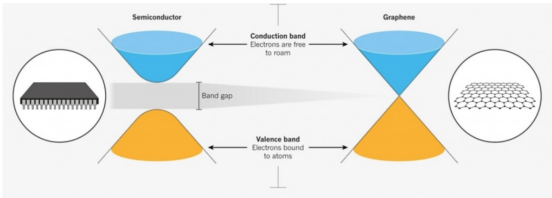
FIGURE 1.3: Energy dispersion in conventional semi-conductors (left panel) compared to the energy dispersion in graphene (right panel). Graphene is seen as a zero gap semi conductor.
