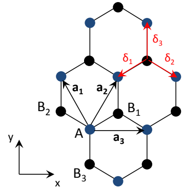
FIGURE 1.5: Tight binding model for graphene honeycomb lattice.
