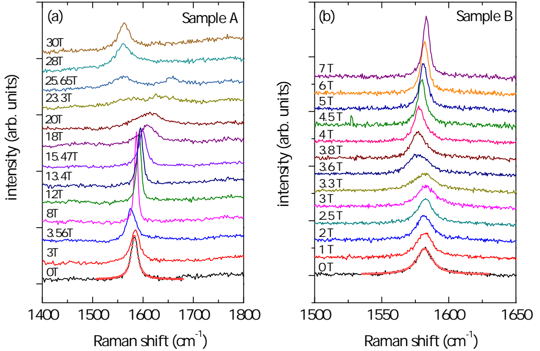
FIGURE 4.4: (a,b) Magneto-Raman scattering spectra in the G band energy range from sample A and B, respectively. In both samples, the G band exhibits strong MPR. The red dots indicate Lorentzian fits of the G band.
