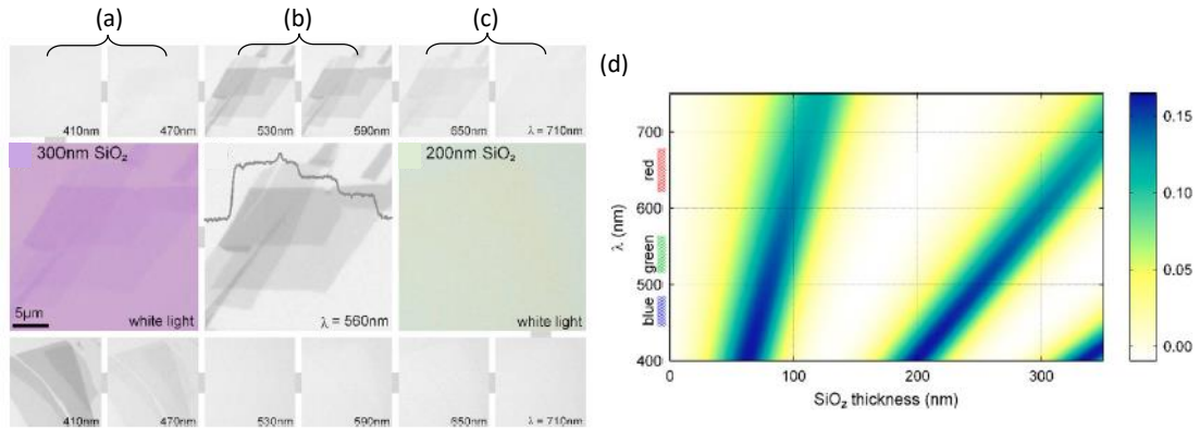
FIGURE 7.2: Optical microscope imaging of graphene flakes. The flakes contain areas of different thickness so that one can see changes in a flake's visibility with increasing numbers of layers. White light illumination on a 300 nm SiO 2 layer in (a), and green light (560 nm) illumination on a 300 nm SiO 2 layer in (b). (c) White light illumination on a 200 nm thick SiO 2 layer. Top and bottom panels in (a-c) show the same flakes but illuminated through various narrow band-pass filters. (d) False color map of the contrast from monolayer graphene as a function of the oxide thickness and the excitation wave-length. Figures were taken from [248].
