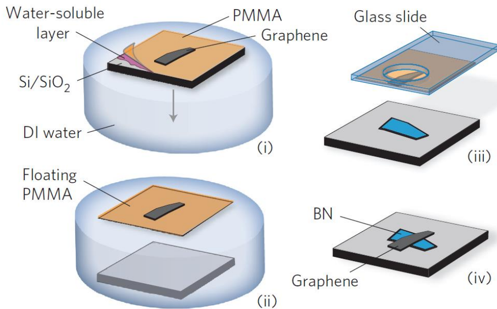
FIGURE 7.1: Four steps process that has been used to fabricate graphene-hBN hetero-structures. Figure taken from [219].
