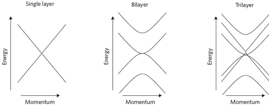
FIGURE 1.7: Band structure of multilayer graphene changes when changing the number of graphene layers on the system [22].
