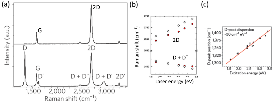
FIGURE 2.5: (a) Two Raman spectra of monolayer graphene. The upper spectrum is taken from a graphene flake with no defects, while the lower spectrum is of highly disordered graphene [84].(b,c) Phonon dispersions as function of the laser excitation energy for the D,2D and D peaks. The red symbols in (b) are for graphene monolayer, while the lozanges are data from graphite [83, 84].
