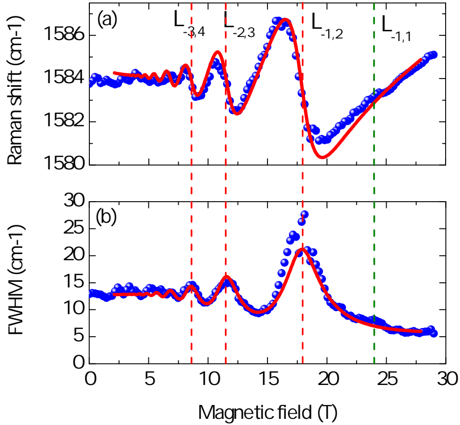
FIGURE 4.17: (a,b) Energy position and FWHM respectively obtained from a single Lorentzian fit of the G band feature as a function of the magnetic field for BG-hBN. The vertical red dashed lines mark the observed resonant magnetic fields for the \Delta|n| = \pm 1 excitations while the green dashed line indicates the L_{-1,1} excitation. The red solid lines are the result of the calculation of the MPR in BG, without considering the L_{-1,1} excitation.
