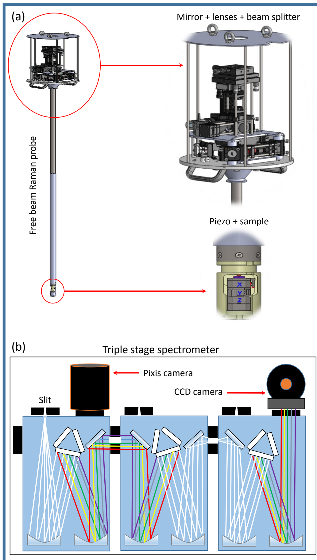
FIGURE 3.3: (a) Free beam probe used for low frequency magneto-Raman measurements. (b) Schematics of the triple stage spectrometer. The triple stagers are in the subtractive mode.
