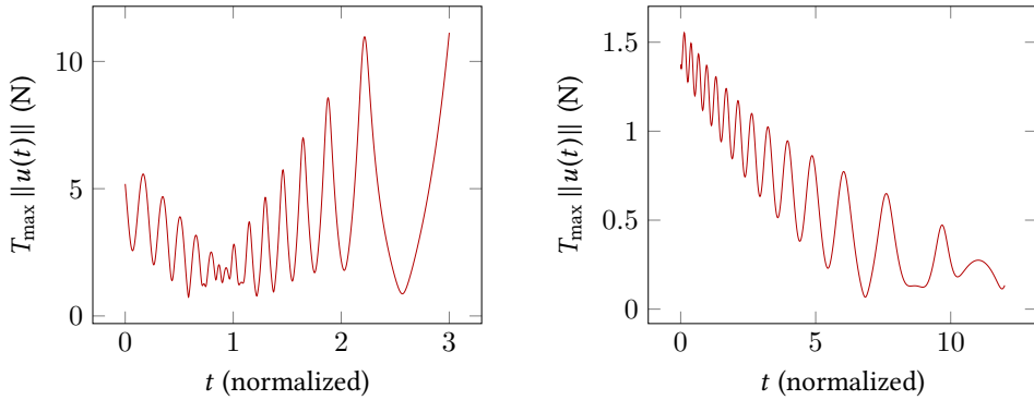
(a) Control of the first controlled part to reach the point belonging to the invariant manifold in the Poincaré map U_1 . The transfer time is fixed to 3.0 in the normalized unit system.
