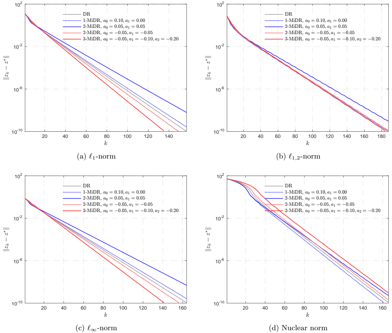
Figure 4.7: Comparison of DR and MiDR for problem \min_{x \in \mathbb{R}^n} R(x) s.t. \mathcal{K}x = \mathcal{K}x_{\text{ob}} with R being \ell_1, \ell_{1,2}, \ell_\infty -norms and nuclear norm. The parameter \gamma in DR algorithm is set to be 1 for all examples.
