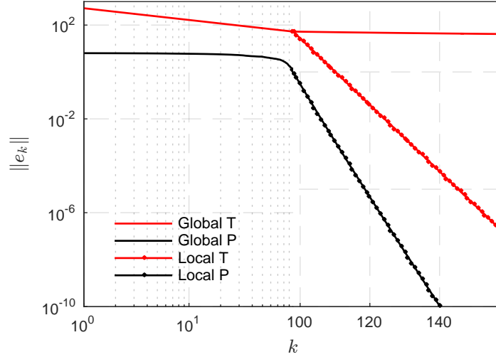
Figure 3.2: Global and local convergence profiles of gradient descent minimizing F with (\underline{\eta}, \bar{\eta}) = (0.8, 1) . The step-size is chosen as \gamma = 1/(2\bar{\eta}) .
