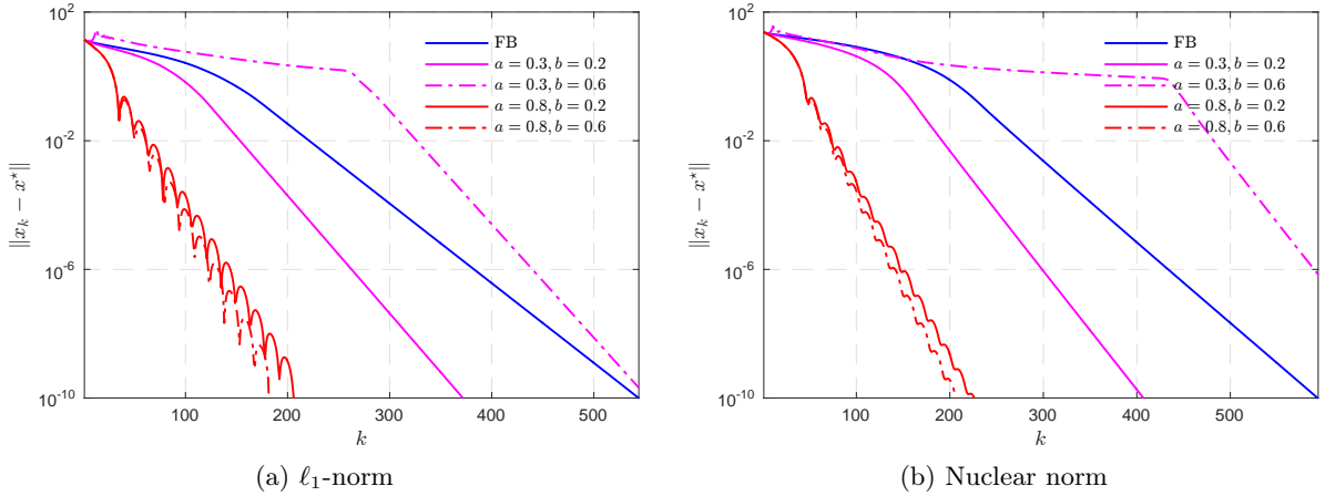
Figure 6.7: Comparisons on the difference between the inertial parameters a_k and b_k , the step-size \gamma is fixed as \beta .
