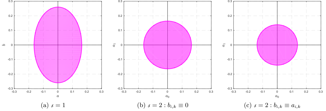
Figure 4.3: Permitted inertial parameters by (4.4.5), where we set \beta = 1, \mu = 0.3, \nu = 0.3, \gamma_k \equiv 0.4\beta and \tau = 10^{-3} .
