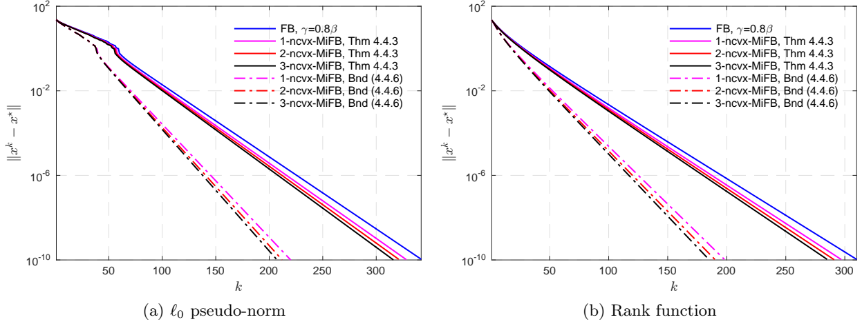
Figure 4.10: Comparison of ncvx-MiFB under different inertial settings. We fix \gamma_k \equiv 0.8\beta for all tests. For the three inertial schemes, the inertial parameters were chosen such that (4.4.5) holds.
