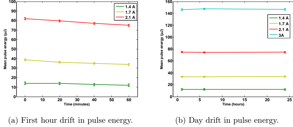
Figure 2.11 – Pulse energy drift measurements.
