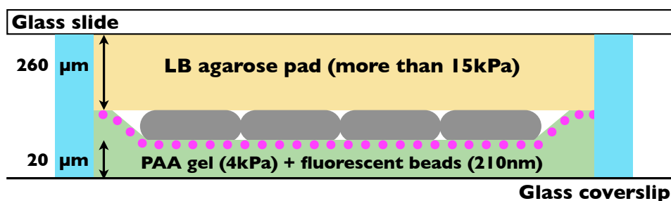
Figure 2.13 – Schematic representation of a TFM sample.
