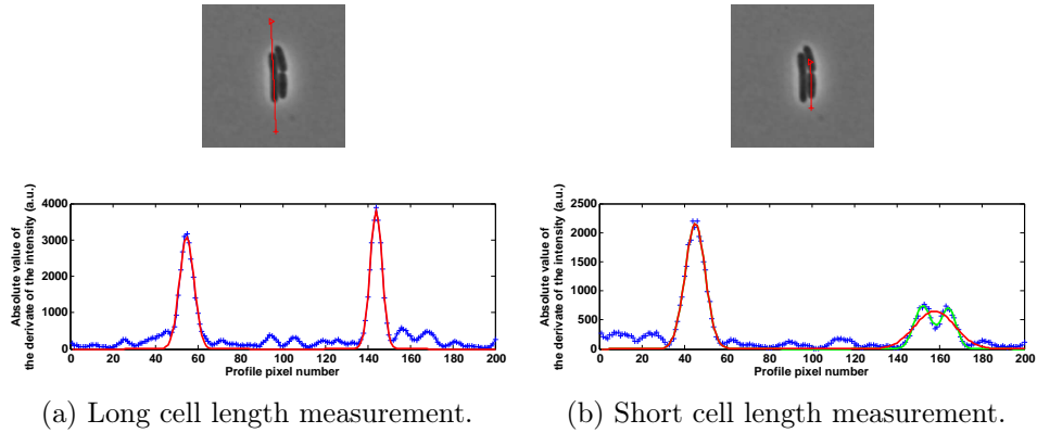
Figure 2.6 – The edges of the cell are determined by fitting the absolute value of the derivative of the intensity profile along the cell main axis by gaussian curves. The preferred fit between one (red) or two (green) gaussian curves is automatically or manually chosen based on variance and fit relevance arguments.
