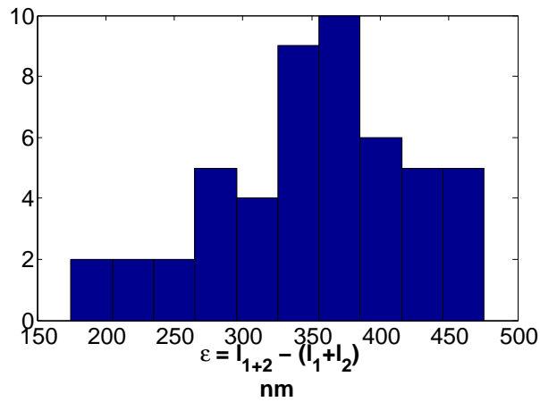
Figure D.2 – Estimation of \epsilon . Histogram of the difference (expressed in nm) between the external pole-to-pole distance l_{1+2} and the sum of individual cell lengths before ablation (in the in-line configuration). 50 experiments are displayed on this histogram.
