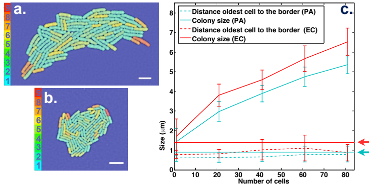
Figure 3.9 – Localization depending on age.
