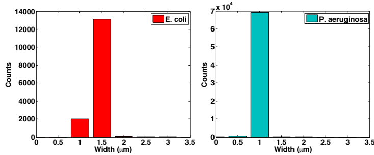
(b) Width distributions.
