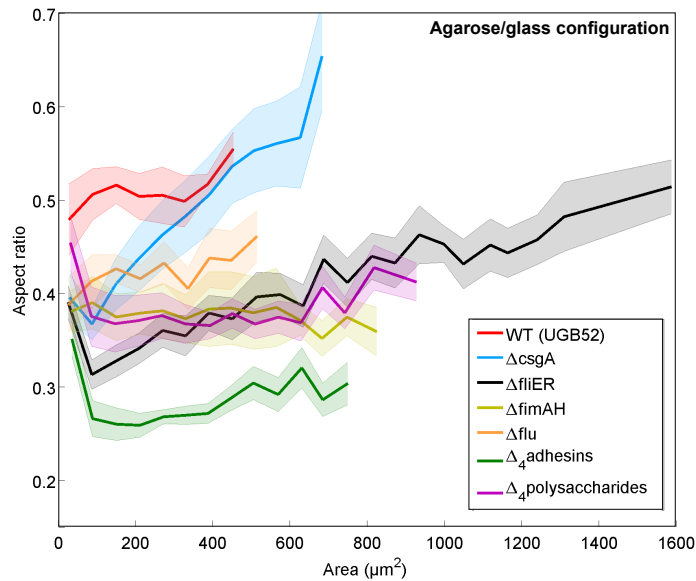
(a) Aspect ratios of different E. coli colonies.
