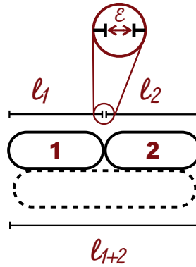
Figure D.1 – Length measurements before the eventual ablation-induced reorganization. The cell to be ablated is represented by a dashed line. Measured lengths refer to the short cells, denoted 1 and 2.
