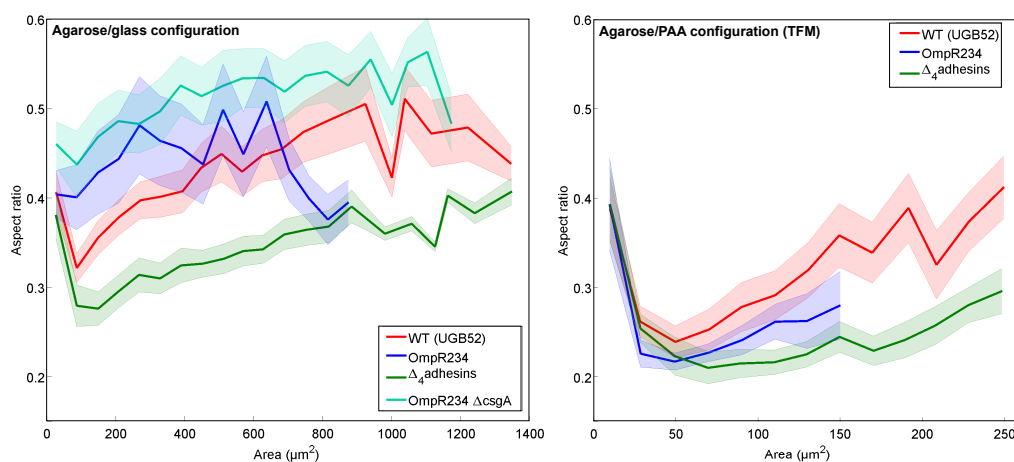
Figure 3.26 – Influence of the expression of curli fibers on the morphology of E. coli colonies grown at 28 °C.
