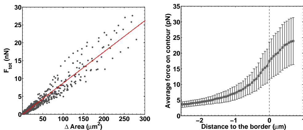
(a) Evolution of the total force.
