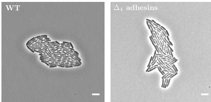
(b) Images of colonies formed by the E. coli WT (left) and \Delta_4\text{adhesins} (right).
