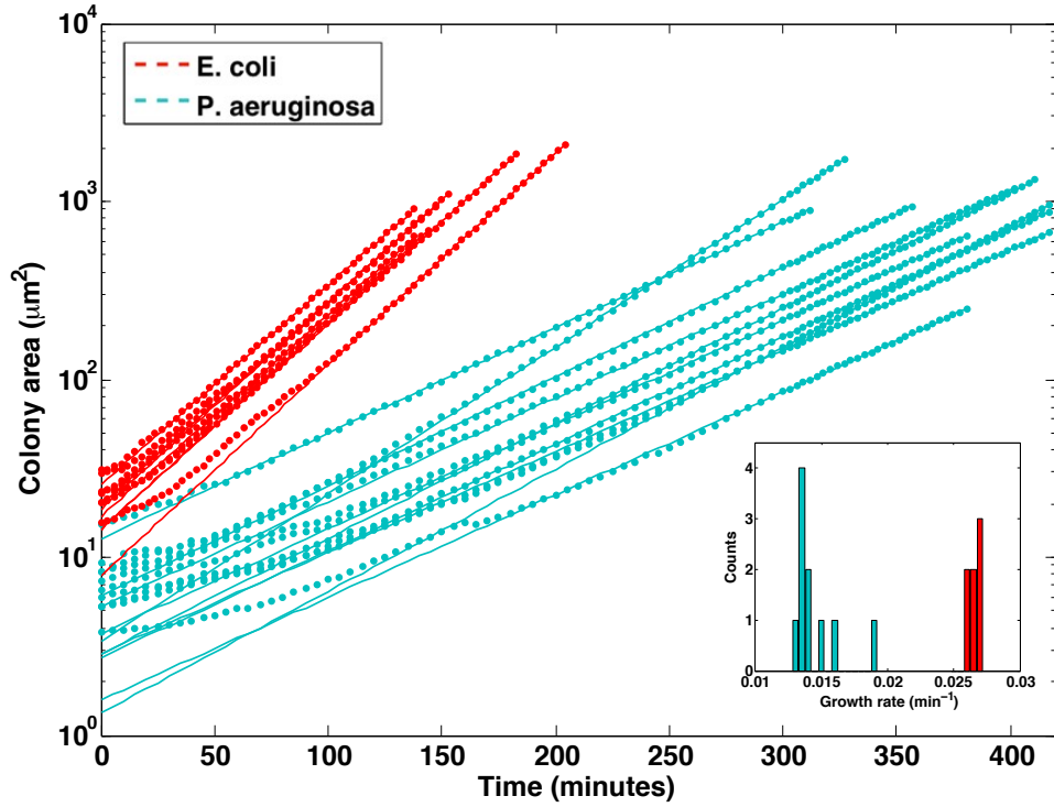
Figure C.1 – Colony area depending on time for E. coli (red) and P. aeruginosa (blue). The colony area \mathcal{A} is represented in log scale, and fitted with an affine relation: \log \mathcal{A} = \alpha t + \beta (all R^2 > 0.99 ). Slopes \alpha define the growth rate of the colony and their distribution is displayed in the inset for each strain. \langle \alpha^{E. coli} \rangle = 0.026 \pm 0.0005 \text{ min}^{-1} and \langle \alpha^{P. aeruginosa} \rangle = 0.014 \pm 0.002 \text{ min}^{-1} , corresponding respectively with characteristic times of 38.5 min and 71.4 min.
