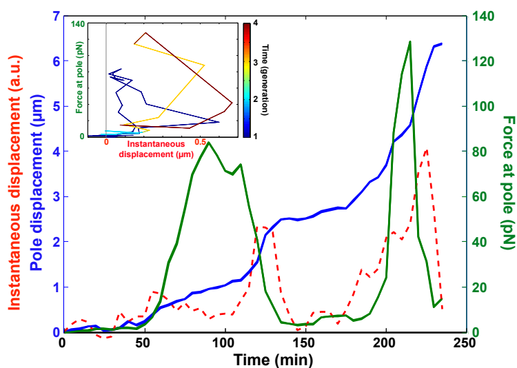
(a) Example of a pole displacement (blue), instantaneous displacement (red) and force (green).
