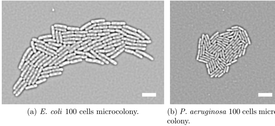
Figure 3.13 – Correlation images (see paragraph 2.1) of microcolonies counting approximately 100 cells for E. coli (left) and P. aeruginosa (right). Scale bar is 5 \mu\text{m} on each image.
