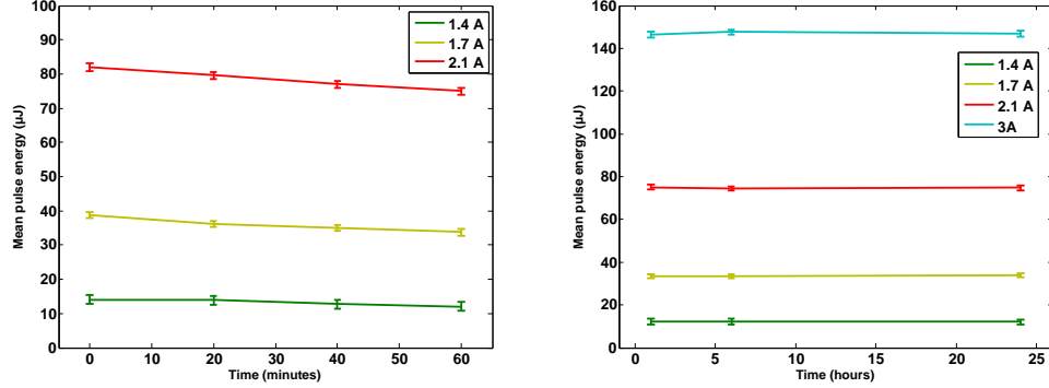
(a) First hour drift in pulse energy.
