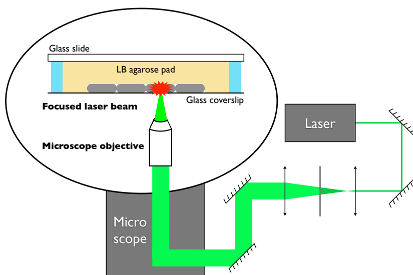
Figure 2.9 – Light path for laser ablation.
