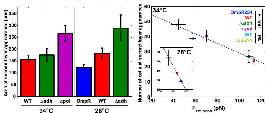
Figure 3.30 – Average surface of the colony at appearance of the second layer for E. coli mutants grown between agarose and polyacrylamide (left panel). The number of cells at appearance of the second layer is linear with the saturation value of the maximal force measured inside the colony. Fits: N_{bact} = -a \cdot F_{max}^{sat} + b , with a = 0.31 \text{ pN}^{-1} and b = 61 at 34^\circ \text{C} ( E. coli and P. aeruginosa ) and a = 1.31 \text{ pN}^{-1} and b = 140 at 28^\circ \text{C} ( E. coli ); R^2=0.99 (see right panel). Error bars on the surfaces or number of cells are the standard errors, error bars on the force saturation are the uncertainty of the fit (95% confidence interval).
