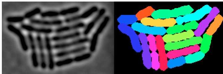
(a) Example of segmentation on an E. coli phase image.
