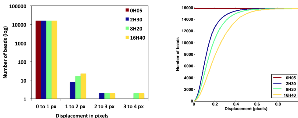
(c) Histogram (counts in log scale) of the displacements sizes depending on time. (d) Cumulative distribution of the displacements depending on time.
