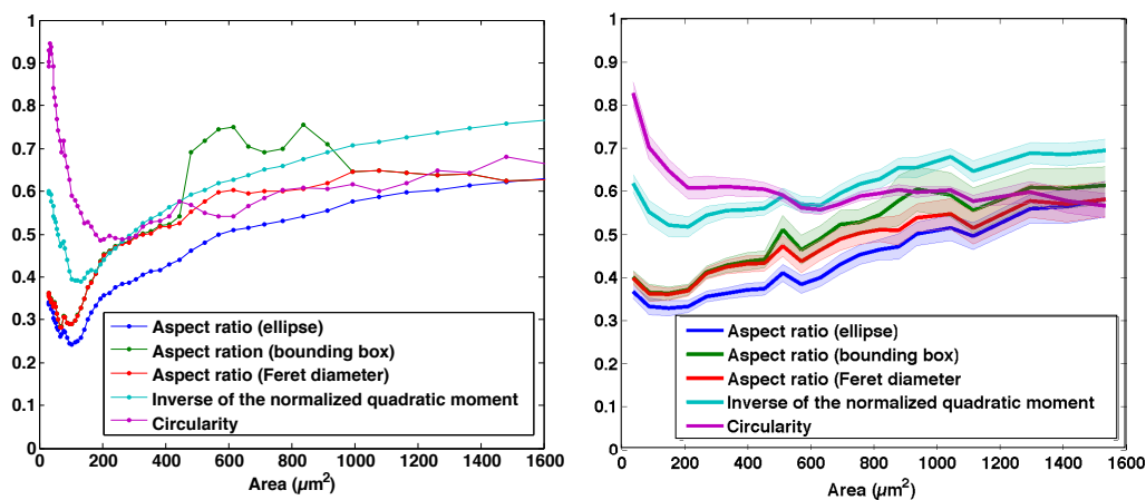
Figure 2.8 – Comparison of the morphological parameters.
