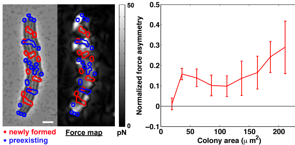
Figure 3.21 – Force asymmetry persists in a developing microcolony. On the left panel, the location of preexisting (blue) and new (red) poles (spatial extension 64 nm in radius) is overlaid on the phase contrast image of the colony and the force map. Scale bar on phase contrast image is 5 \mu\text{m} . Right panel shows the evolution of the normalized asymmetry in force A_N(F) , defined by equation 3.6, as a function of the colony area. Positive values mean that the maximal force at preexisting poles is higher than the maximal force at newly formed poles. The presented curve is an average over 13 colony growths. Bin size is 25 \mu\text{m}^2 and error bars represent the standard errors.
