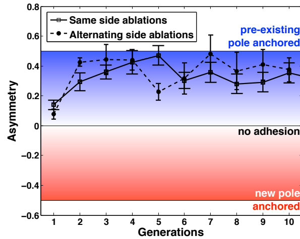
Figure 3.5 – Oriented asymmetry parameter at each generation during the single cell ablation experiments. If the asymmetry is positive/negative (blue/red area), the preexisting/newly formed pole is more anchored to the substrate. If it is 0, there is either no anchoring or a symmetric anchoring. Results are displayed for same side ablation experiments (squares and full line, N=9) and for alternating side ablation experiments (disks and dashed line, N=5). Error bars represent the standard errors. Both experiments indicated a preferential anchorage of the preexisting pole to the substrate.
