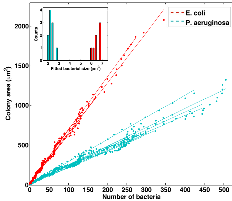
Figure C.2 – Linear fits of the colony area depending on the number of bacteria in the colony for E. coli (red) and P. aeruginosa (blue). The distribution of the slopes, corresponding to the average bacterial surface, are displayed in the inset (bin size is 0.2 \mu\text{m}^2 ). 7 colony growths were considered for E. coli and 10 for P. aeruginosa .
