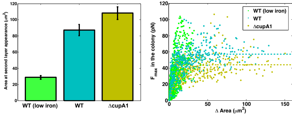
(a) Adhesion strength set the area of 2D spreading.
