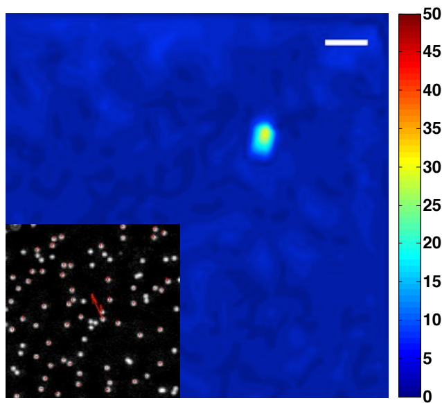
Figure 2.16 – Example of sudden bead displacement.
