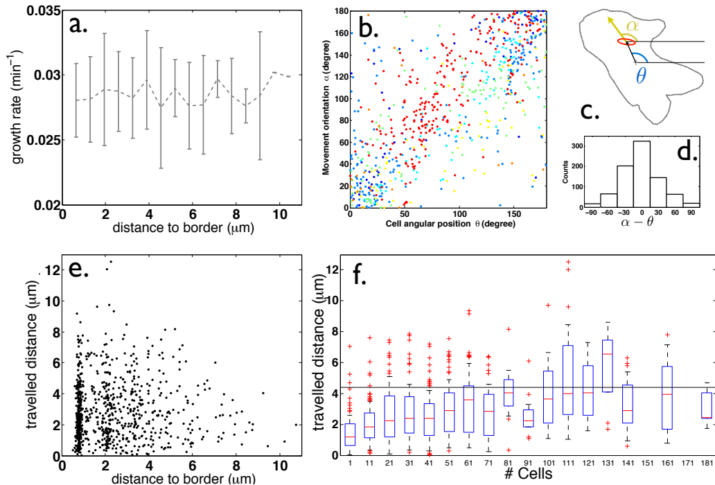
Figure 3.10 – Evidence of radial pushing in E. coli microcolonies.
