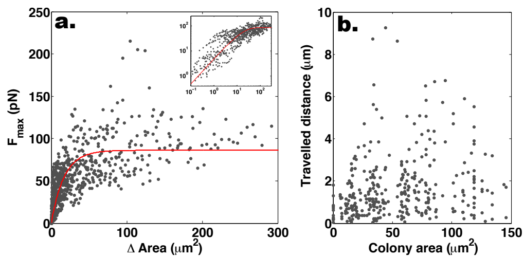
Figure 3.18 – (a) The maximal force observed inside the colony increases with the variation of area of the colony and then, saturates. Grey dots are extracted from measurements on 13 E. coli wild-type colonies growing at 28 °C. Each dot is a frame. The red line is the fitted trend: F_{\max}(A) = F_{\max}^{\text{sat}} \cdot (1 - e^{-\frac{A}{A_0}}) ( R^2 = 0.6 ), with F_{\max}^{\text{sat}} = 86 (83; 90) pN and \frac{1}{A_0} = 0.059 (0.052; 0.066) \mu\text{m}^{-2} i.e. A_0 = 17 \mu\text{m}^2 . The inset represents the data and the fit in log-scale. (b) Evolution of the travelled distance of bacteria over their cycle depending on the area of the colony. Each point stand for one bacterium. No data is provided for large areas since cells had not completed their cycle before the end of the acquisition.
