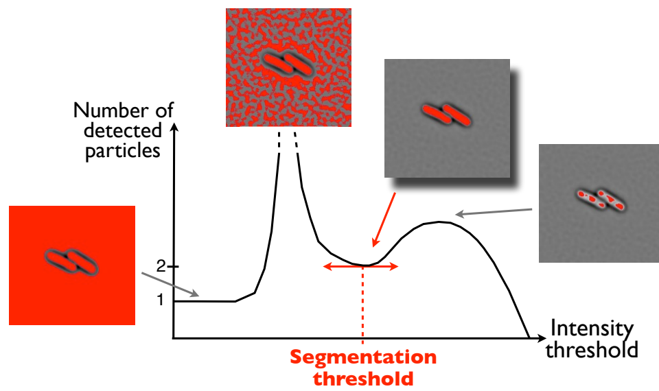
Figure 2.2 – Segmentation on correlation images.
