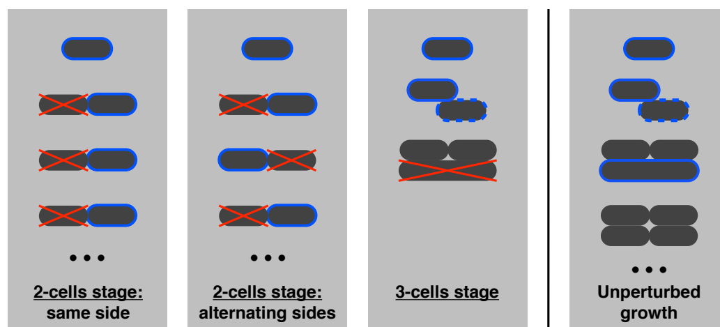
Figure 2.12 – Summary of ablation rules for the different experiments. The three ablation experiment procedures are displayed to be compared to a regular unperturbed growth (right panel). For each situation, time increases when going down and in between each step, a division event occurred. When displayed, the next cell to divide is circled with a blue solid line. When 2 divisions should theoretically be simultaneous but are slightly desynchronized due to intrinsic noise, the cell with a delayed division is circled with a blue dashed line. The ablated cells are crossed in red.
