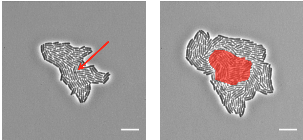
Figure 3.27 – Appearance of the second layer.
