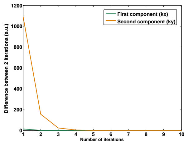
Figure 2.15 – Representative example of the convergence of the continuous mode of the stress field for the two components of the Fourier space.
