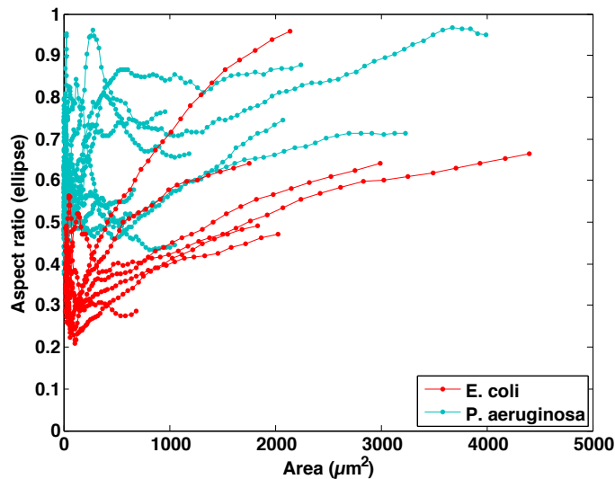
Figure 3.12 – Aspect ratio for E. coli and P. aeruginosa colonies. Aspect ratios of the colony as a function of the colony area, for E. coli (7 colony growths, red) and for P. aeruginosa (10 colony growths, blue).
