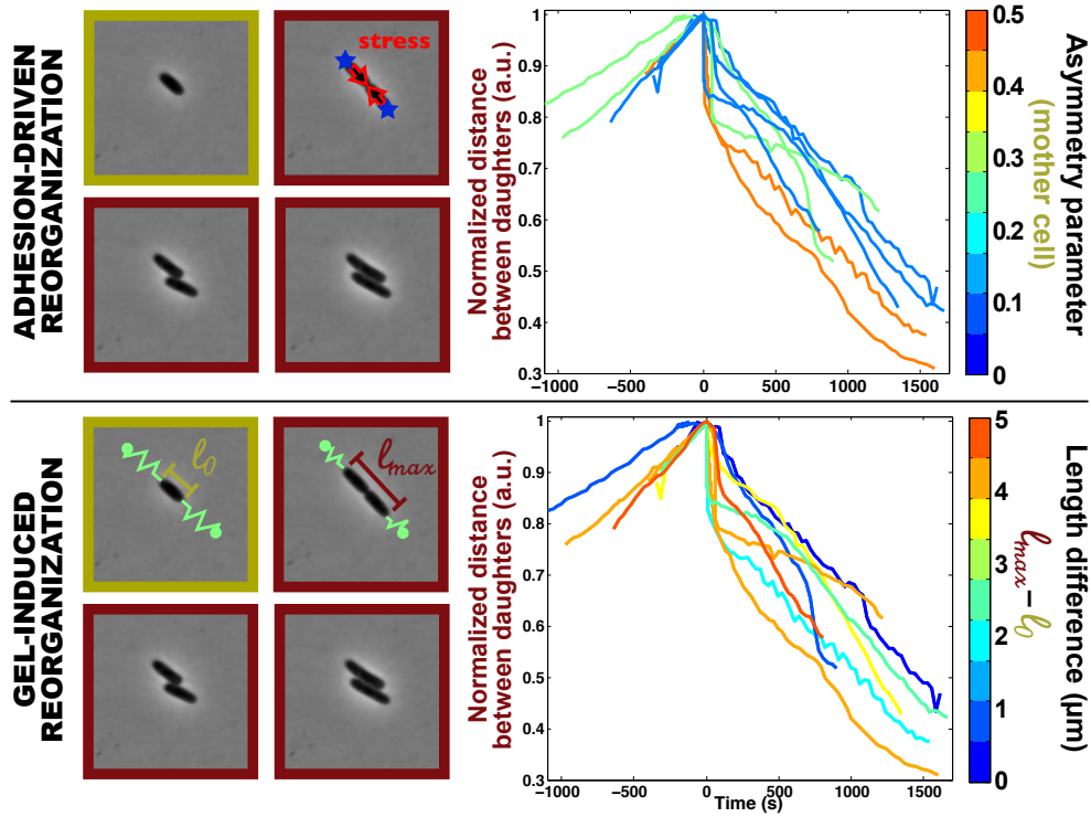
Figure 3.7 – Two hypotheses are analyzed to explain the reorganization: an adhesion-driven mechanism (upper panel) and a gel-induced mechanism (lower panel). For both cases, the normalized distance between the 2 daughter cells depending on time is displayed for all experiments. For each of the 7 experiments, the corresponding curve is color-coded depending on the asymmetry parameter of the mother cell (upper panel) or depending on the cell extension l_{max} - l_0 , l_0 being the length of the initial cell and l_{max} the sum of the lengths of the daughter cells just before reorganization (lengths displayed on the left lower panel).
