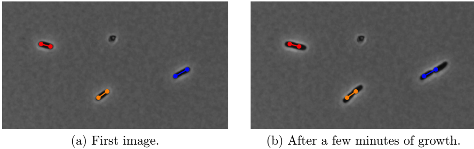
Figure 3.1 – The colored dumb-bells on the initial image stand for position of cells before growth. After a few minutes of growth, bacteria appear to have elongated asymmetrically compared to their initial position. All the images were recentered to correct for potential drifts on a fixed feature (here on the small particle).
