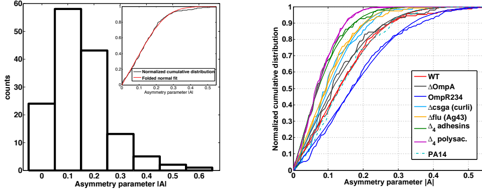
(a) Histogram of asymmetries for the wild-type E. coli strain (WT, N=146). (b) Normalized cumulative distributions of asymmetries.
