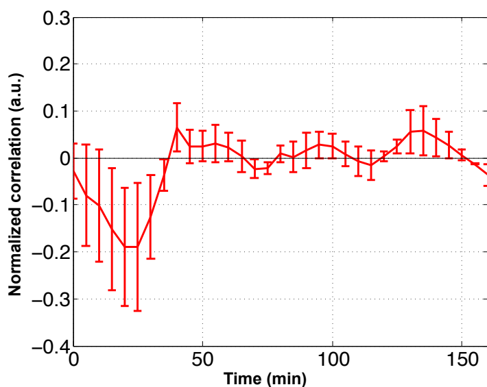
(b) Correlation between the instantaneous displacement and the variation of force.
