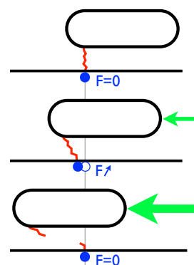
Figure 3.19 – Bond rupture scenario. F represents the force applied on the gel, measured from its deformation.
