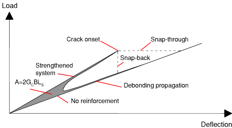
Figure 4.13: Load–deflection curve for a reinforced TPB beam
