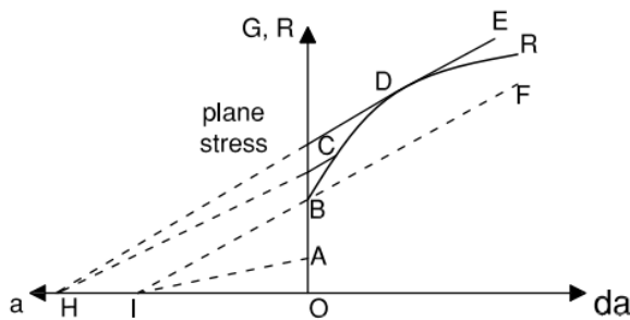
Figure 2.12: Energetic criterion in plane stress state
