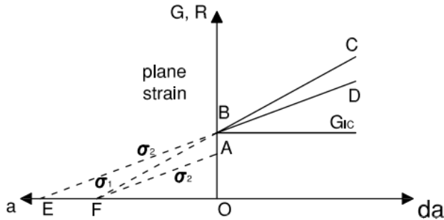
Figure 2.11: Energetic criterion in plane strain state
