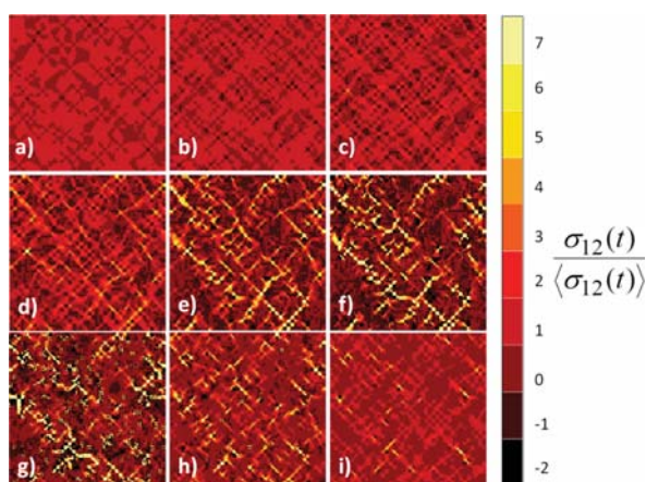
Figure 12. Maps of \frac{\sigma_{12}(t)}{\langle \sigma_{12}(t) \rangle} calculated taking G_r = 10^{-3}G_g and \sigma = 2 . From left to right, the dimensionless time t/\tau_{\max} and average macroscopic stress \langle \sigma_{12}(t)/\tau_{\max} \rangle are equal to, respectively, (a) (3 \times 10^{-4}, 0.9\epsilon_0 G_g) ; (b) (10^{-2}, 0.7\epsilon_0 G_g) ; (c) (0.1, 0.45\epsilon_0 G_g) ; (d) (1, 0.2\epsilon_0 G_g) ; (e) (10^1, 0.05\epsilon_0 G_g) ; (f) (40, 0.01\epsilon_0 G_g) ; (g) (4 \times 10^2, 0.0002\epsilon_0 G_g) ; (h) (1 \times 10^4, 5.10^{-5}\epsilon_0 G_g) ; (i) (10^6, 2.10^{-5}\epsilon_0 G_g) .
