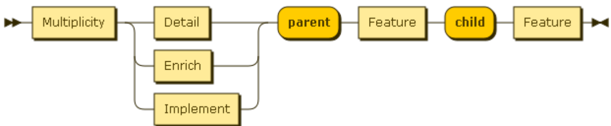
FIGURE A.8 : DirectedBinaryRelationship
