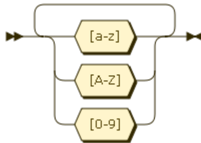
FIGURE A.25 : String
