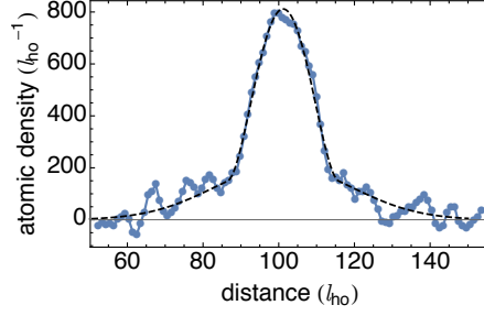
Figure 2.13: Doubly integrated density profile of a relatively hot bosonic cloud. Blue line: experimental profile. Dashed black line: bimodal fit of the density distribution. Here, the temperature extracted from the thermal cloud width is 233 nK, while the condensed fraction is \sim 50\% , corresponding to a temperature of 238 nK.
