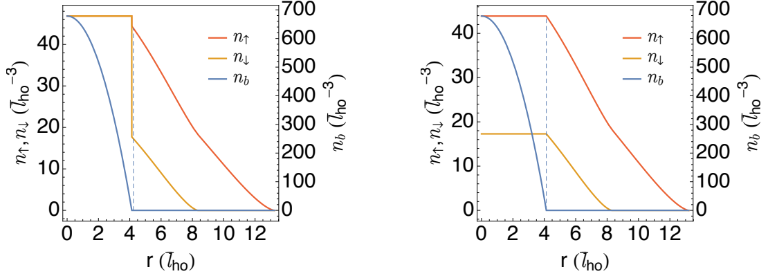
(a) Critical situation (i): the superfluid (with n_{\uparrow} = n_{\downarrow} ) occupies the whole core and does not expand out of it.
