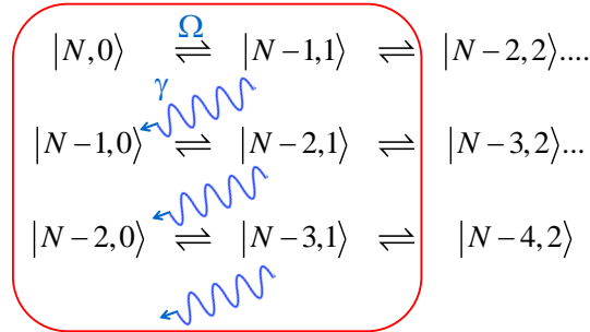
Figure 3.18: Radiative cascade of the center of mass motion. In |N, n\rangle , N (resp. n ) refers to the center of mass (resp. relative) motion of the two clouds (see text).
