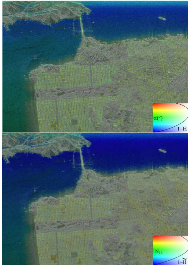
Figure 14: Polarimetric colored representation using first classical parameters Entropy and alpha, and then new proposed parameters scattering diversity and surface scattering fraction.
