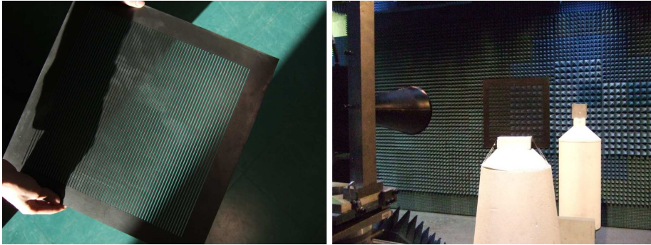
Figure 18: Pictures of the experimental setup to validate the new calibration method principle
