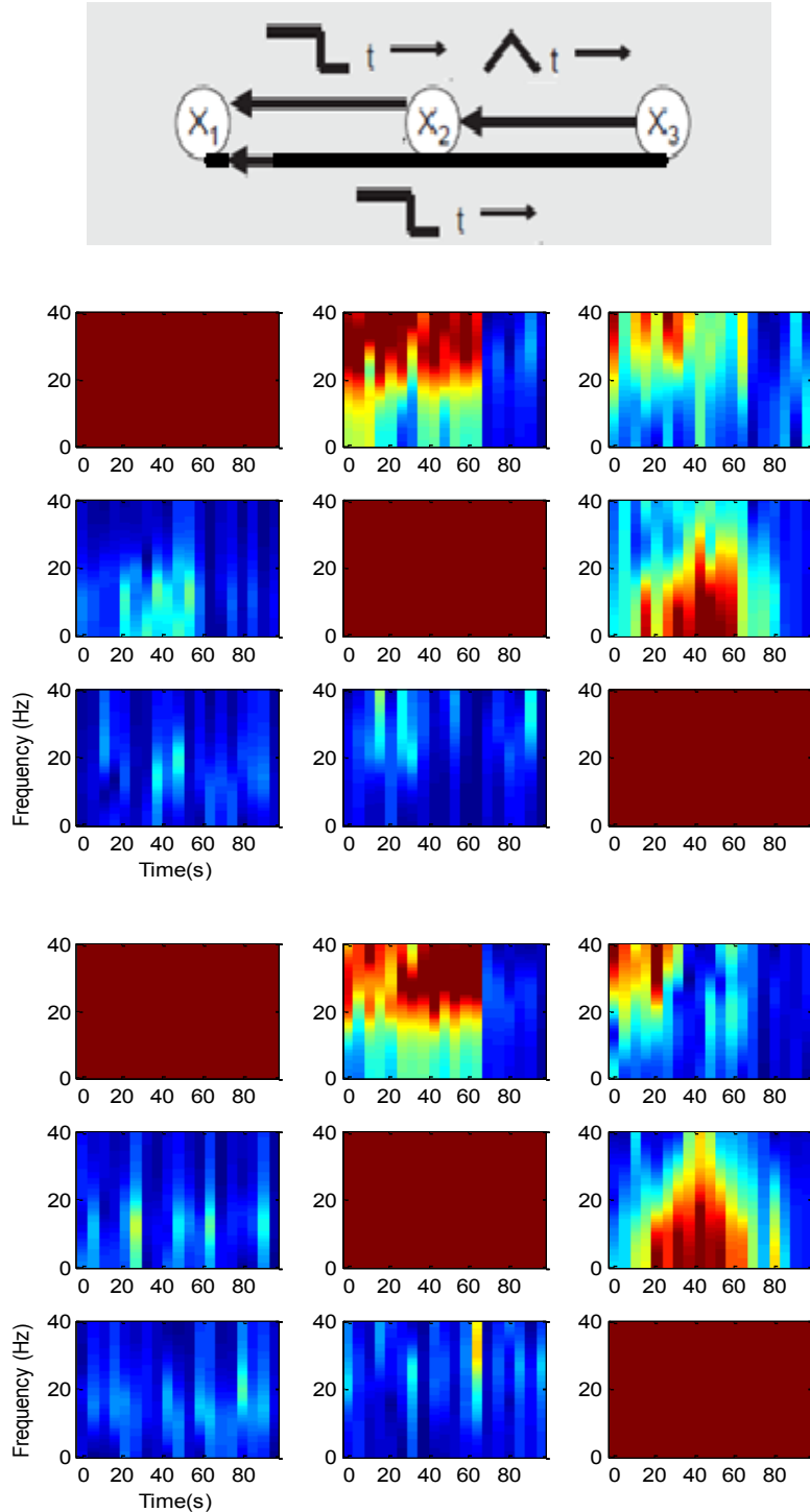
Figure 4.7: (Top) Description of the LNS system; (Middle) DTF results; (Bottom) PDC results
