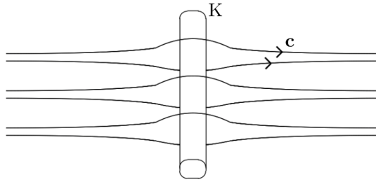
Figure 3.2: Vector field \mathbf{c} avoiding laterally a tube K
