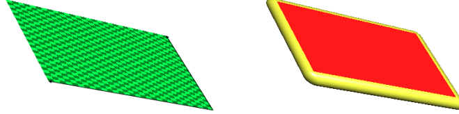
Figure 2.3: Simplex S and \{x : \text{dist}_\phi(x, S) < \langle \mathbf{M}\boldsymbol{\nu}, \boldsymbol{\nu} \rangle^{\frac{1}{2}}\}
