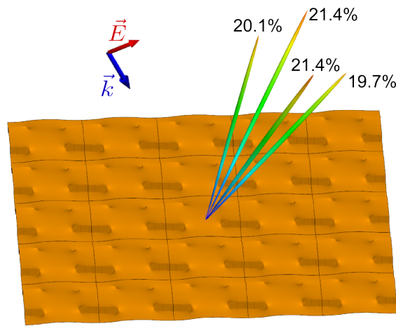
FIGURE 5.23: Far-field pattern of the designed phase grating with a 25^\circ incident plane wave
