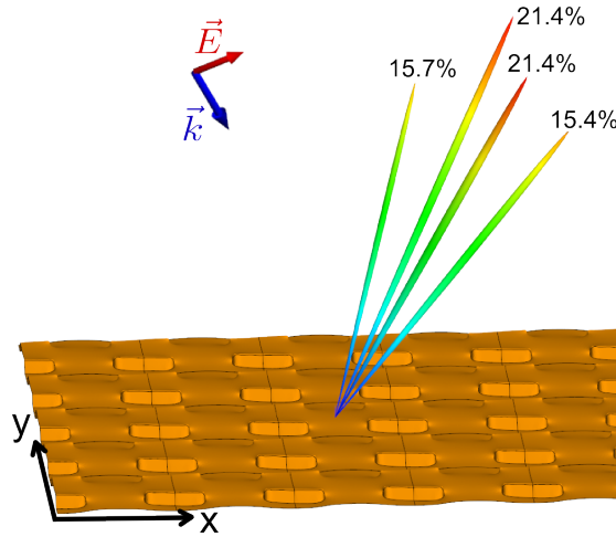
FIGURE 5.32: Far-field pattern generated by the grating with oblique edges
