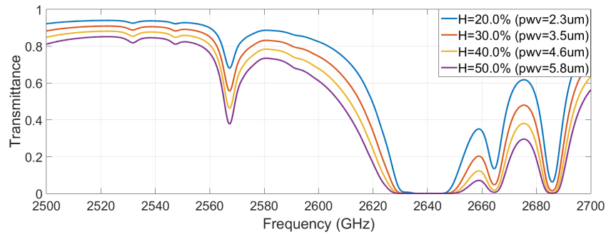
FIGURE 4.21: Atmospheric transmittance for a 50\text{ cm} optical path at 25\text{ }^{\circ}\text{C}
