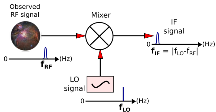
FIGURE 2.2: Principle of the heterodyne detection
