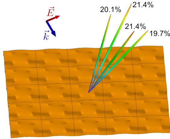
FIGURE 5.23: Far-field pattern of the designed phase grating with a 25° incident plane wave
