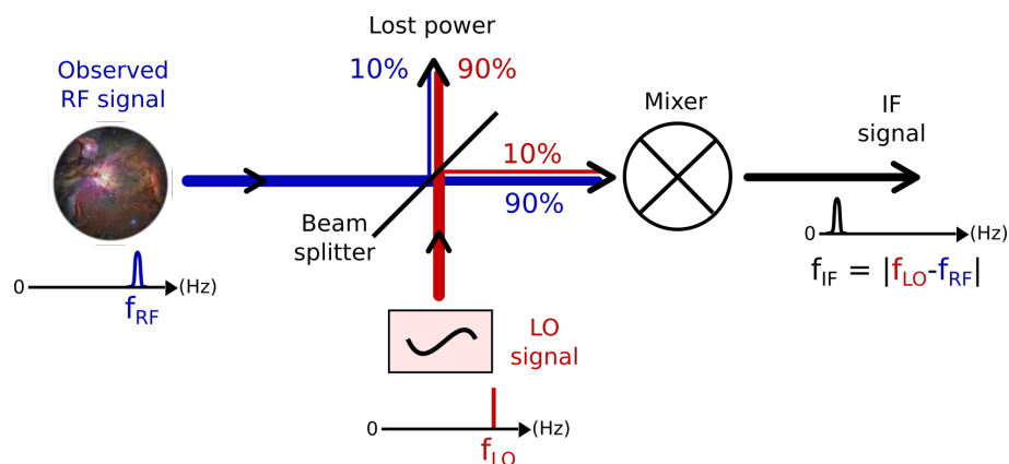
FIGURE 4.1: Schematic showing the down-conversion of the RF signal's frequency and the use of a beam splitter
