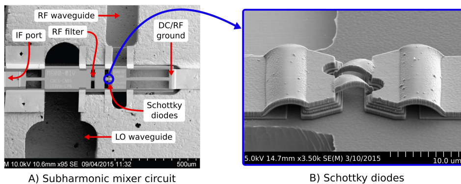
FIGURE 2.6: SEM picture of a LERMA-LPN 600 GHz subharmonic mixer (A), and of an anti-parallel pair of Schottky diodes (B) (Credits: Alain Maestrini)
