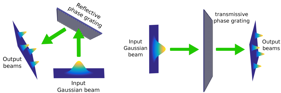
FIGURE 5.1: Reflective and transmissive phase gratings
