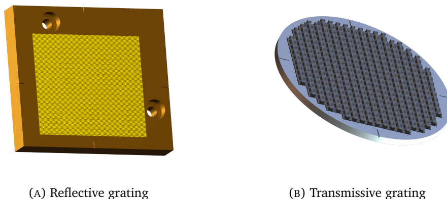
FIGURE 5.25: Final 3D designs of the 2 phase grating prototypes
