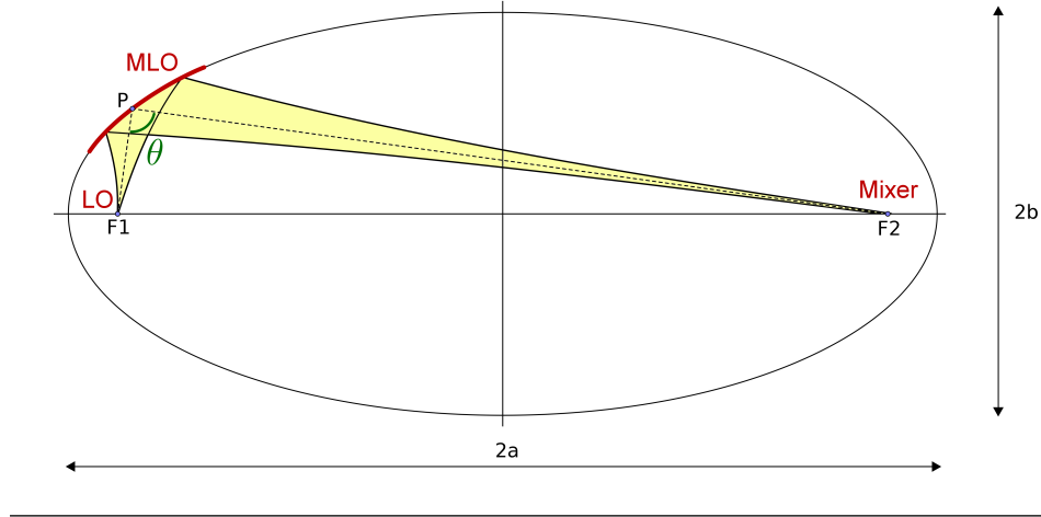
FIGURE 4.11: Schematic of the ellipsoidal mirror (MLO)
