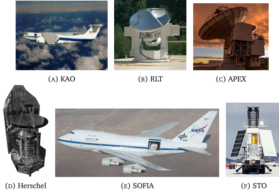
FIGURE 2.1: Pictures of different heterodyne receivers operating above 1 THz
