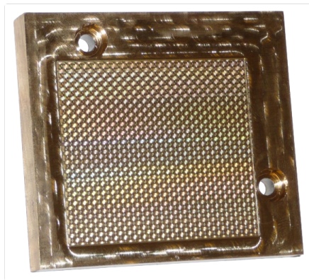
FIGURE 5.26: Manufactured reflective phase grating
