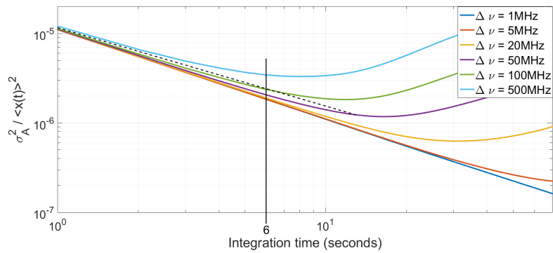
FIGURE 3.21: Spectral Allan variance of the receiver with a 1400 GHz multiplier chain LO
