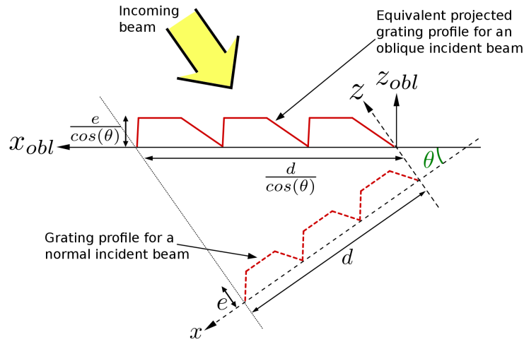
FIGURE 5.17: Example of a projected grating's relief for an oblique incident beam
