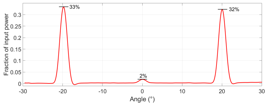
FIGURE 5.10: Angle and power of the output beams
