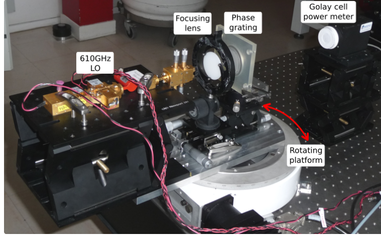
FIGURE 5.35: Set-up of the experiment to test the transmissive grating
