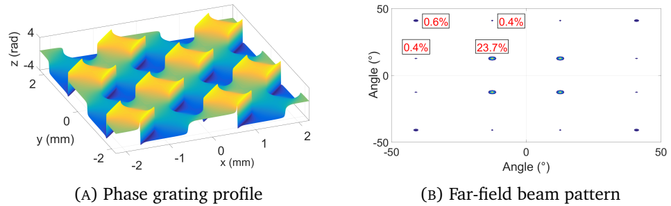
FIGURE 5.14: Phase grating generating the far-field pattern of fig. 5.12c
