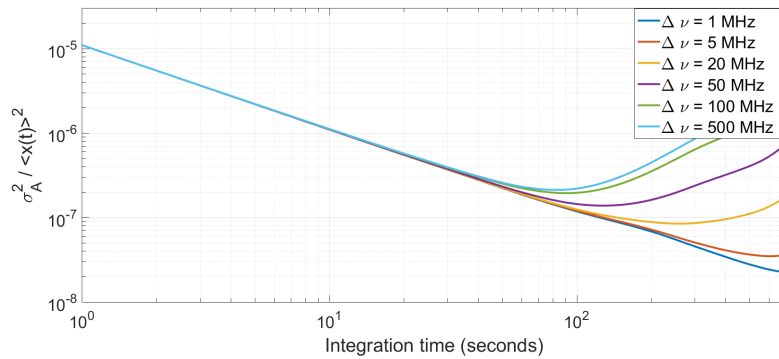
FIGURE 3.18: Spectral Allan variance of the receiver with a 600 GHz multiplier chain LO
