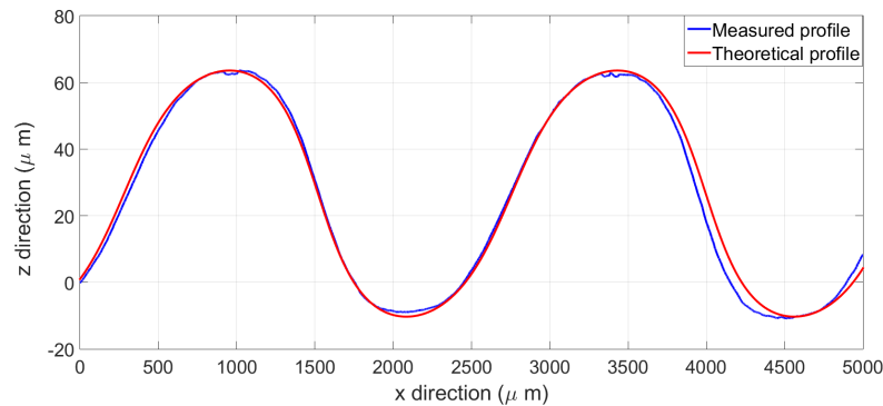
FIGURE 5.28: x scan of the grating's surface
