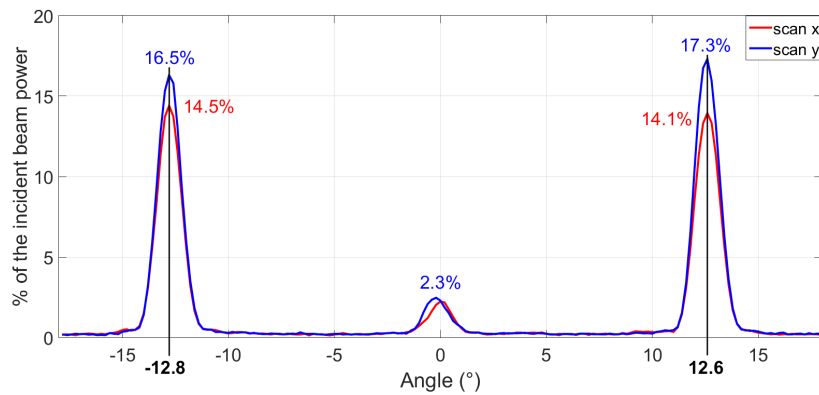
FIGURE 5.36: Power and position of the 4 beams created by the transmissive grating
