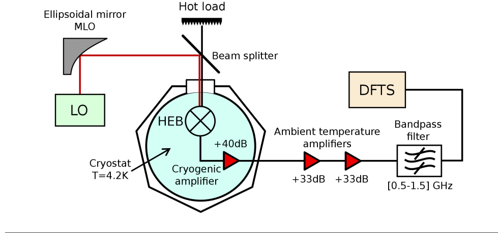
FIGURE 3.6: Schematic of our heterodyne receiver set-up
