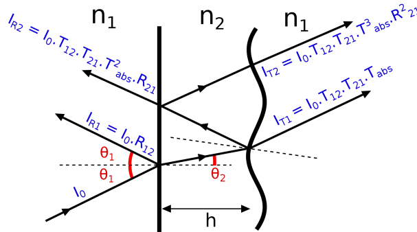
FIGURE 5.24: Intensities transmitted and reflected at the grating's interfaces
