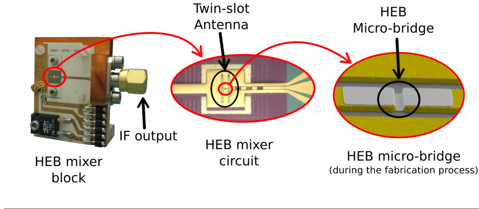
FIGURE 2.8: Pictures of a HEB (Credits: Gregory Gay)
