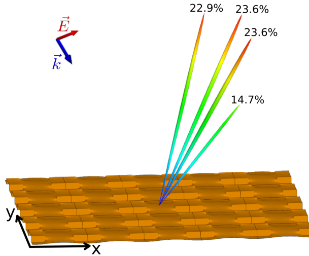
FIGURE 5.21: Far-field pattern of the designed phase grating with a 25° incident plane wave
