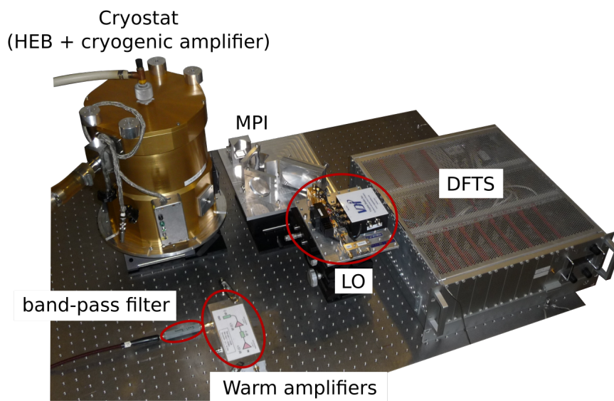
FIGURE 2.14: Picture of our heterodyne receiver
