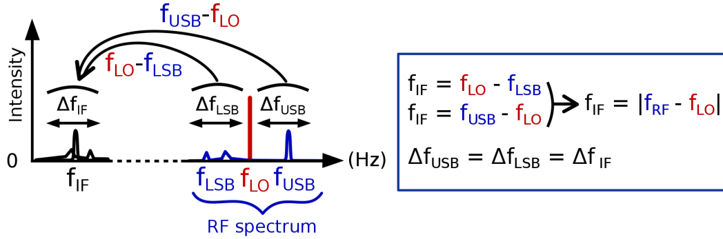
FIGURE 2.5: Down-conversion of the RF side bands
