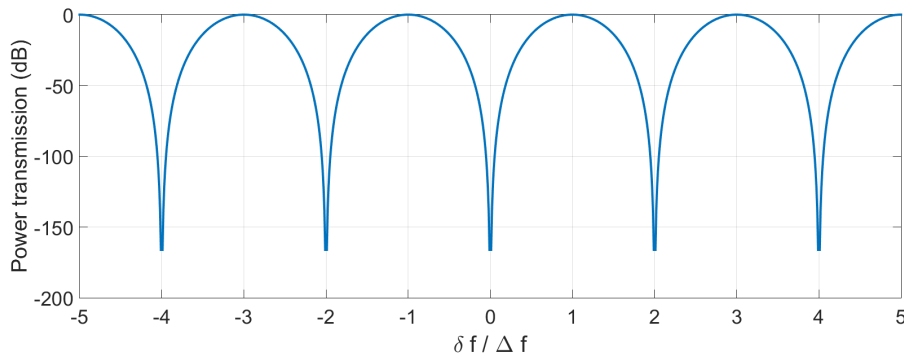
FIGURE 4.8: Bandwidth of the MPI for the horizontal component of the RF signal
