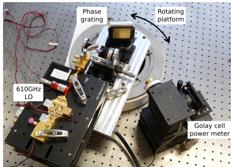
FIGURE 5.33: Set-up of the experiment to measure the efficiency of the reflective phase grating
