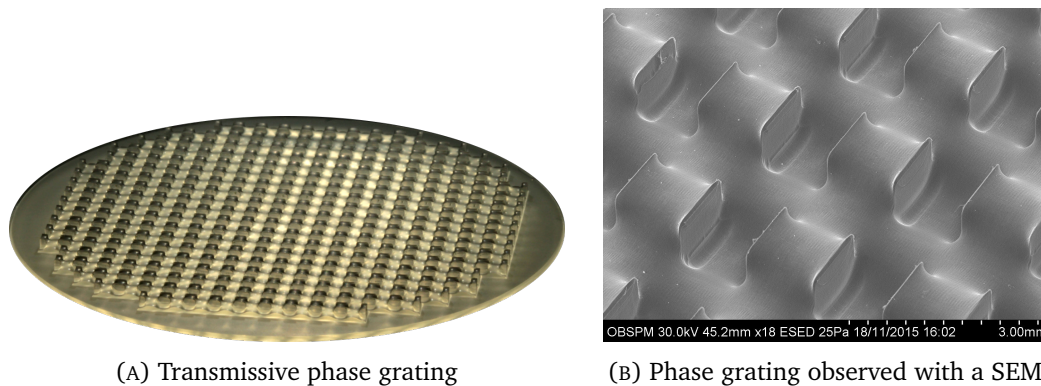
FIGURE 5.30: Pictures of the transmissive phase grating, made of TPX ®
