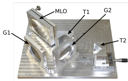
FIGURE 2.12: Picture of a MPI designed at the Observatory of Paris
