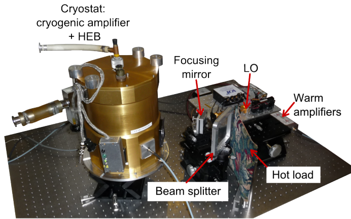
FIGURE 3.16: Picture of the experiment to measure the stability of the LO and HEB mixer
