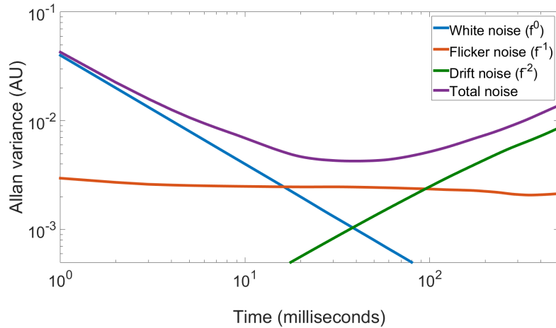
FIGURE 3.3: Allan variance of the 3 noises signals (logarithmic scale)
