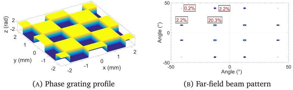
FIGURE 5.13: Phase grating generating the far-field pattern of figs. 5.12a and 5.12b
