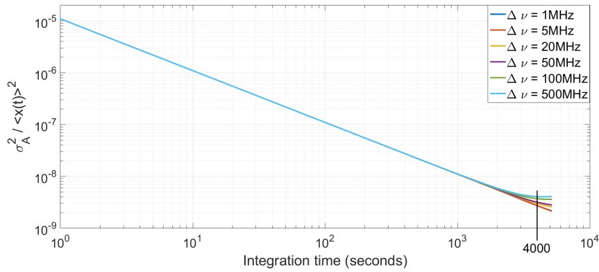
FIGURE 3.11: Spectral Allan variance for different spectral distances
