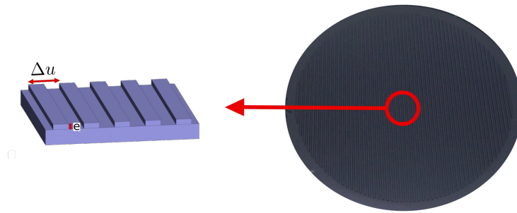
FIGURE 5.5: HRFZ Silicon Dammann grating from Tydex optics
