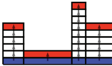
FIGURE 1. A Kakutani–Rokhlin partition
