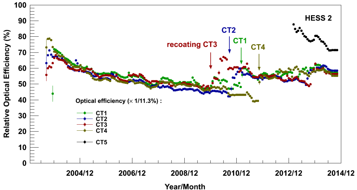
Figure 2.2: H.E.S.S.' optical efficiency as a function of time. From the start of the experiment up to 2010, a global decline of the optical efficiency can be noted, which is to be expected from the wear of the instrument. In 2010, the re-aluminisation of the mirrors improved the optical efficiency. The different peaks in the distributions, the most important one visible in 2006, correspond to cleaning campaigns of the PMTs and cones. In 2012 the curves are more grouped due to the implementation of a new muon reconstruction for the calibration. Concerning the optical efficiency of H.E.S.S. II, it drops faster than that of H.E.S.S. I and the bumps observed come from several realignements of the mirrors.
