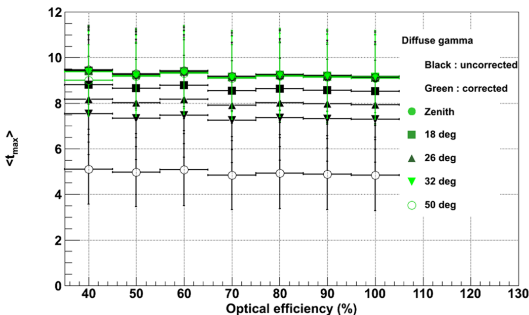
Figure 5.4: Effect of zenith correction on the mean value of MDH ( \langle t_{max} \rangle in the figure) for simulated diffuse gamma and all optical efficiencies. Before correction (in black), the mean value of MDH is different for each zenith angle. After correction (in green) they are superimposed.
