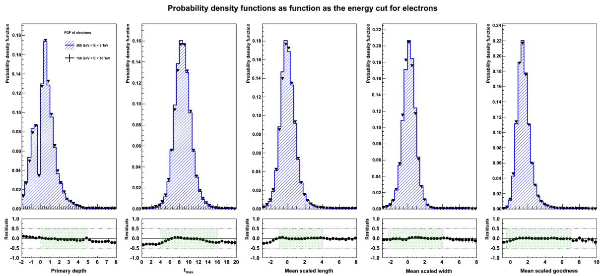
Figure E.2: PDFs for electrons in different energy domains.
