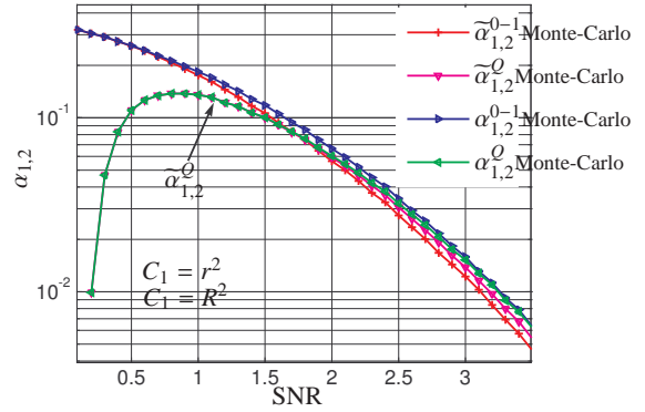
Figure 4.7: Comparison between \tilde{\alpha}_{1,2}^{0-1} and \tilde{\alpha}_{1,2}^O for Geometry 3.
