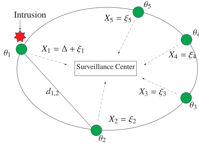
Figure 3.1: Localization of an intruder in a WSN with a monitoring center. The i -th sensor has the geographic location \theta_i .
