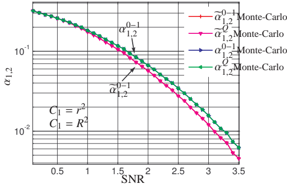
Figure 4.6: Comparison between \tilde{\alpha}_{1,2}^{0-1} and \tilde{\alpha}_{1,2}^O for Geometry 2.
