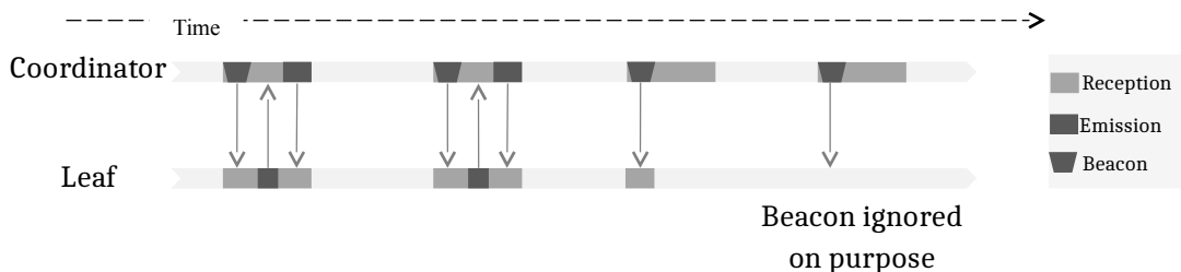
Figure 6.10: Avoid skipping beacons if data is present at coordinator.
