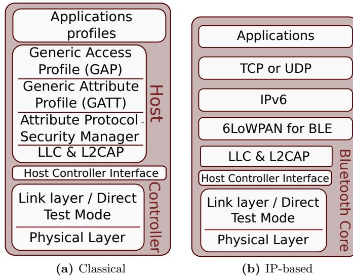
Figure 2.15: BLE Stacks
