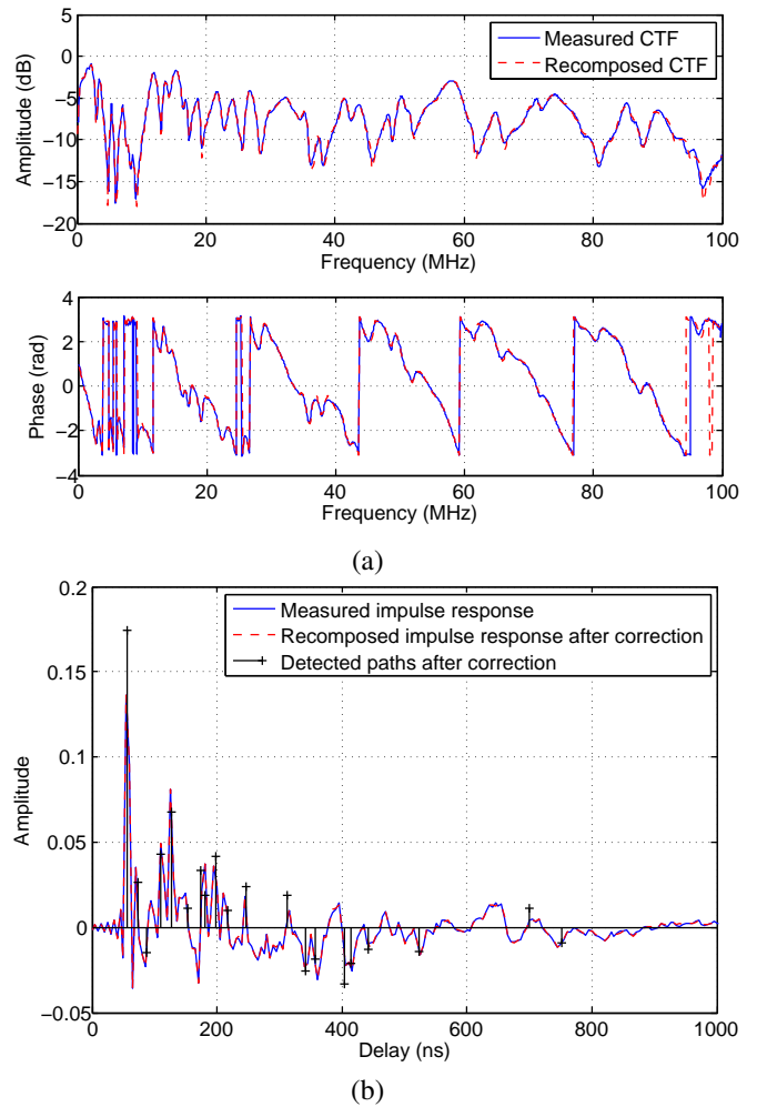
Fig. 6. Application of the MP algorithm on a measurement taken from a home network. CTF (a) and CIR (b).
