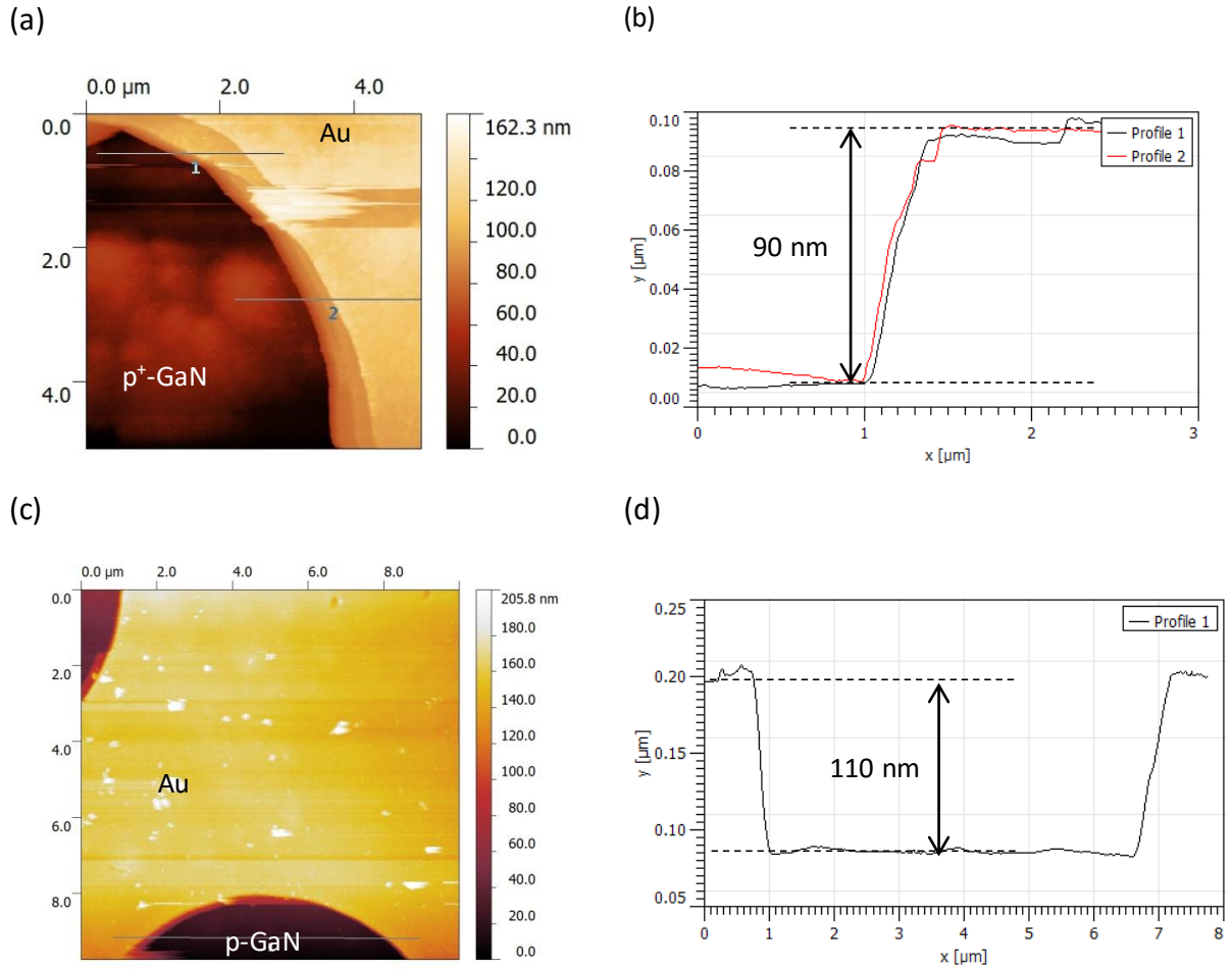
Figure 43 : (a) Constant tunneling current STM topographical image of GaN and Au contact of Seoul 4A sample. (b) profile across the Au contact edge. I_t = 0,5 \text{ nA} and V_g = 2 \text{ V} . Multiple step shape of the Au edge might be due to multiple tip shape. (c) 10 \times 10 \text{ } \mu\text{m}^2 AFM image of the Seoul 4A sample. (d) Cross section along the scan line indicated in (c).
