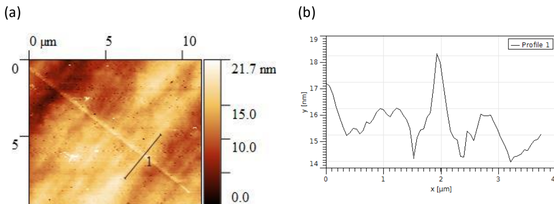
Figure 59 : AFM characterisation of the STM patterned p++-type GaN surface (sample 7Ad_1). (a) Image of the tip-induced patterned line (patterning parameters V_g = -6V and I_t = 20 nA, total exposure time 1 minute). (b) Cross section along the line.
