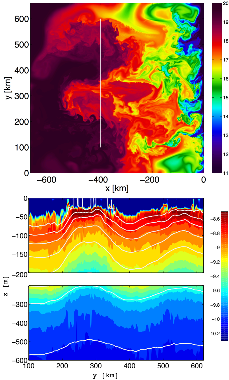
Figure 2.12: Top: Instantaneous SST in the \Delta x = 750 m idealized California current simulation of Capet et al. (2008f). Bottom: Cross section of Ertel potential vorticity ( m^{-1} s^{-1} ) in logarithmic scale, with superimposed isopycnals (white lines) along the meridional section represented in top panel with a white segment. Note the different vertical scales for the [-200 \ 0] and [-600 \ -200] m depth ranges.
