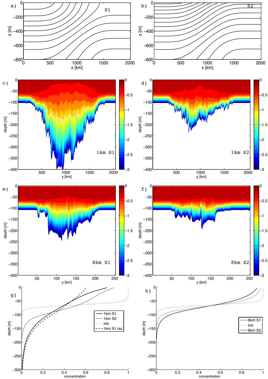
Figure 2.13: a-f): y-z section of initial density (a,b; contour interval is 0.25 \text{ kg m}^{-3} ) and tracer concentration (c-f, log scale) after 30 days of spindown for two baroclinically unstable flows S1 (left, weak stratification) and S2 (right, moderate stratification) with the same mean meridional density gradient. g-h): Horizontally averaged tracer profiles after 30 days at 1km (left) and 8 km resolution for the different experiments. The initial distribution is also shown. In g) tracer distribution is also shown for an experiment using a rotated lateral diffusion operator that minimizes diapycnal mixing (Lemarié et al., 2012) (S1 iso).
