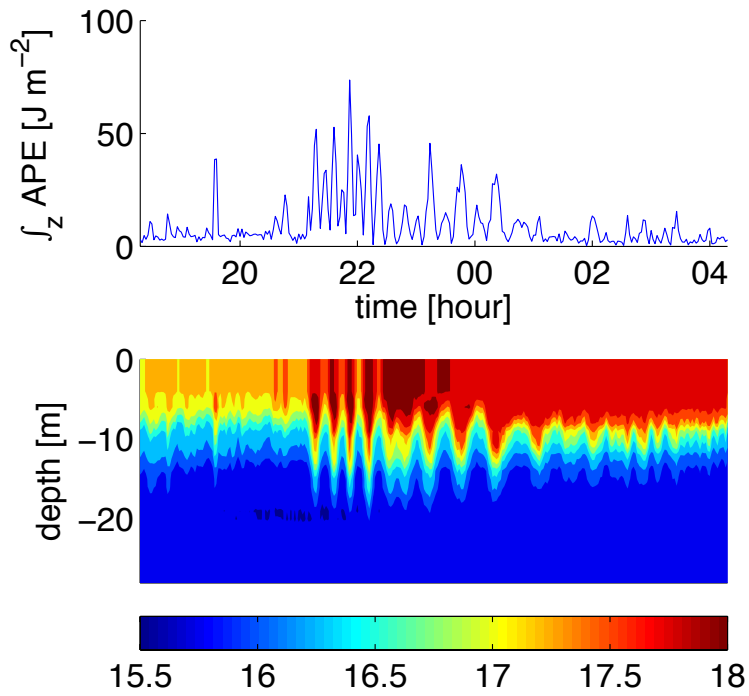
FIG. 12. Time series of available potential energy (top) and temperature vertical profiles at M28 from 24 Feb. 18.20PM to 25 Feb. 4.20AM. during the period of clear IGW activity contributing to the mixing estimates in Sec. 4b). The x-axis scale is identical for the two panels.
