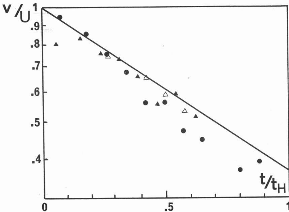
Fig.12 :The decay of the vortex couple. ● B = 1\text{ T} , translation velocity; ▲ B = 0.5\text{ T} , translation velocity; △ B = 0.5\text{ T} , velocity at the couple center divided by 4 (obtained from photographic traces). The theoretical decay is represented by a full line.
