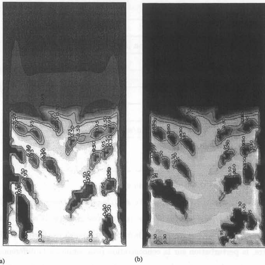
Figure 4-8: Cartes de concentration correspondant au (a) cas 3 Cb_{\max} = 18.42 , Cb_{\min} = -5.10 et (b) cas 10 Cb_{\max} = 16.31 , Cb_{\min} = -2.1 , t=15 min. Isovaleurs \phi = 0.3; 0.5; 0.95 .
