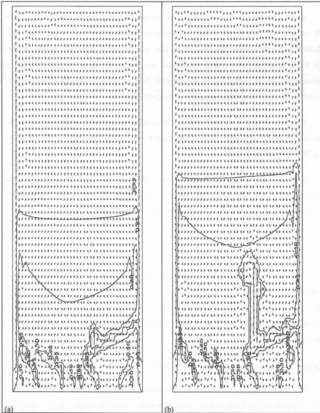
Figure 4-19: Champ de vitesses, grand domaine, cas 8. a) t=15 min ( v_{\max} = 19 mm/sec). b) t=20 min ( v_{\max} = 7.1 mm/sec). Isovaleurs \phi = 0.5; 0.95 .
